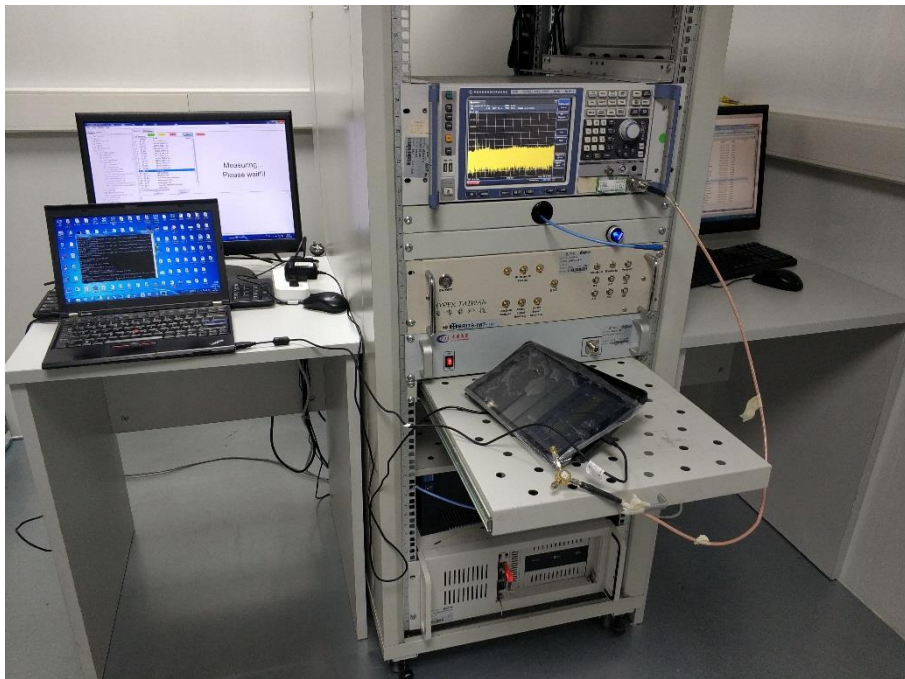
Conducted Test-BT/BLE
