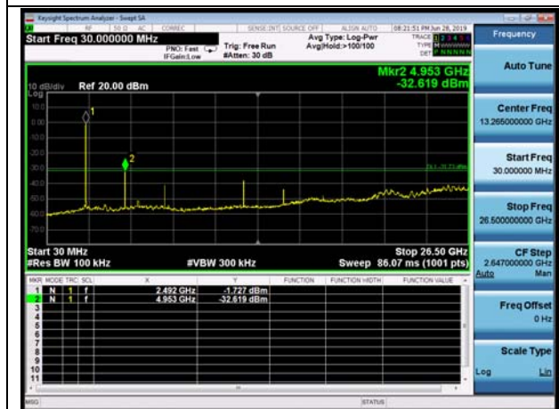
BLE CH39 30MHz to 26.5GHz
