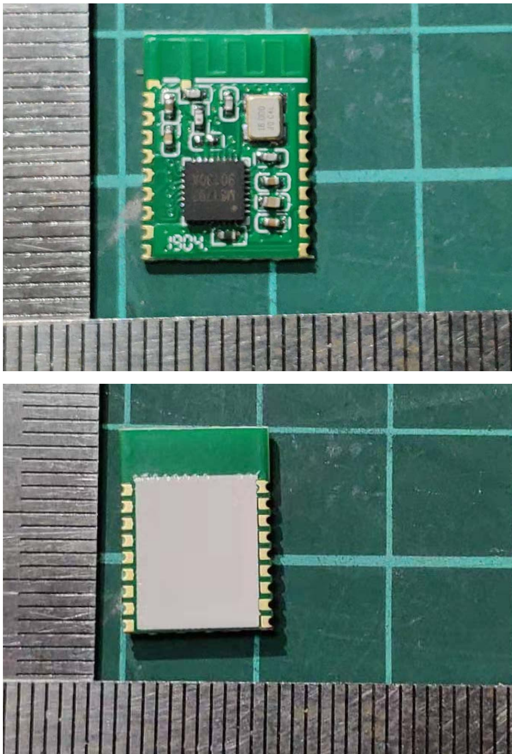
Picture 1 EUT
