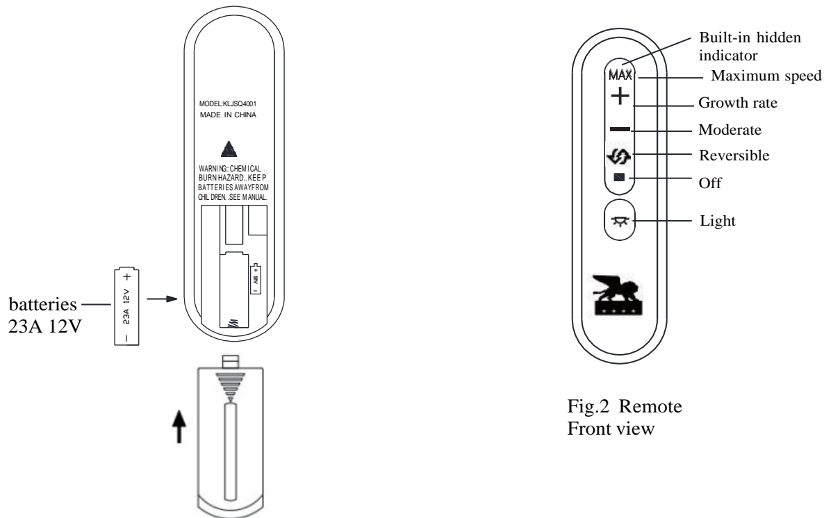
Fig.1 Inserting battery Rear view
