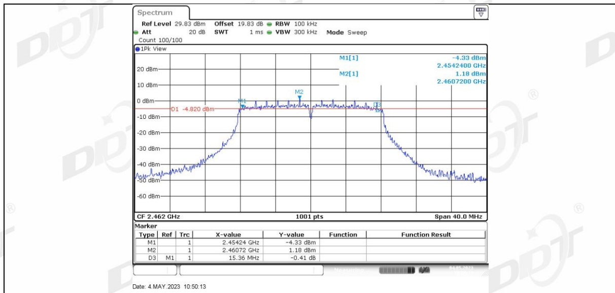
11G Ant2 2462
