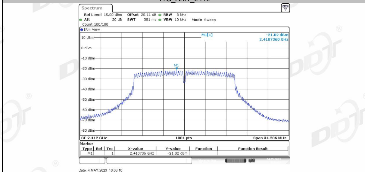
11G Ant2 2412
