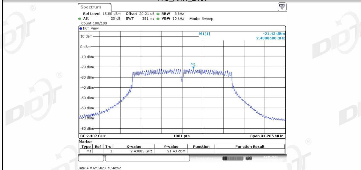
11G Ant2 2437
