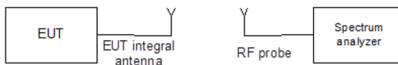
Figure 7.2.1 Occupied bandwidth test setup
