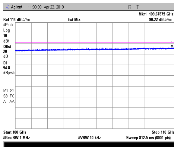
Plot 7.4.7 Spurious emission measurements in 100 – 110 GHz range (continued)
