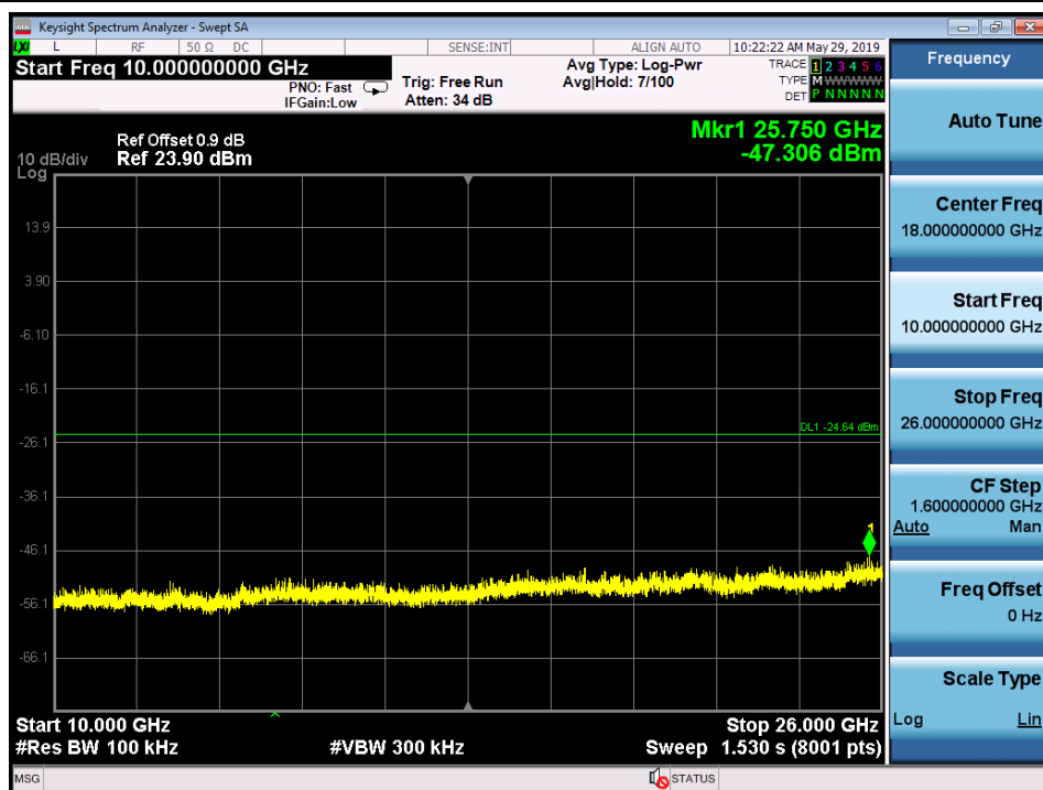
RF Conducted Spurious Emissions 2DH5 2480
