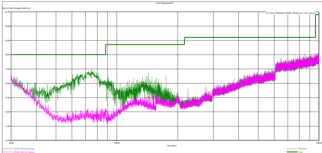
Figure 1 - Radiated Emissions Data Plot, 30M-1GHz, Receive mode
