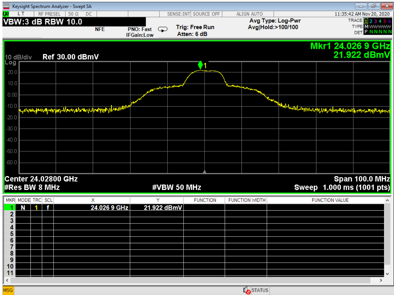
Figure 5 - Analyzer Measurement – Fundamental, Channel Low
