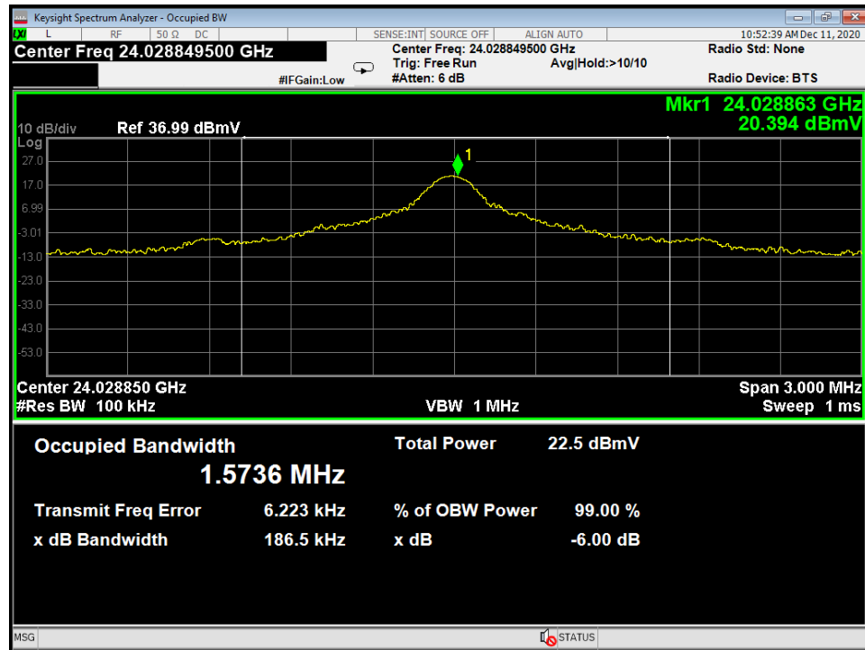
Figure 16 – Occupied Bandwidth, Low channel
