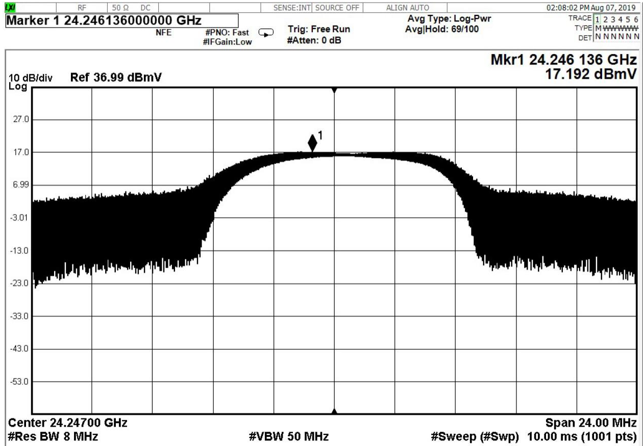
Figure 7 - Analyzer Measurement – Fundamental, Channel High
