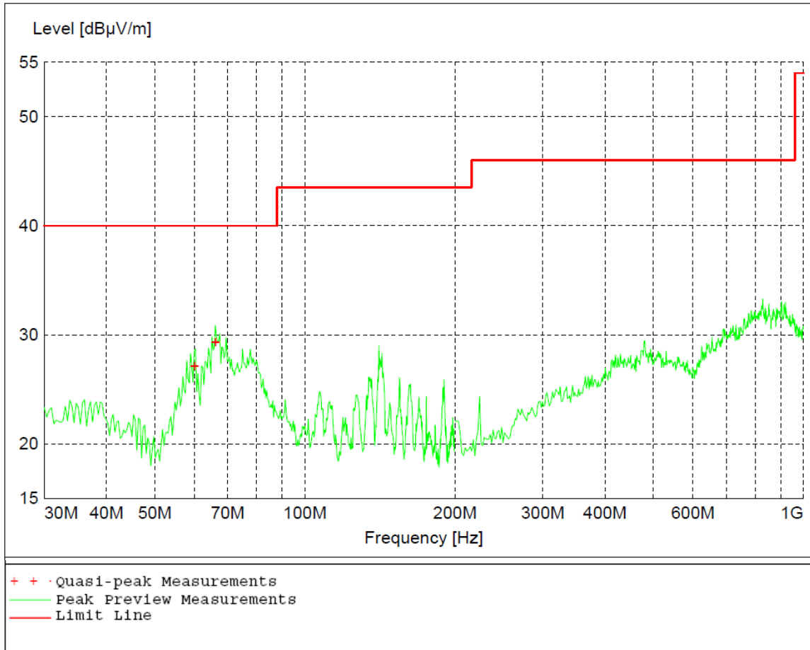
Figure 4 - Radiated Emissions Data Plot, 30M-1GHz, High Channel
