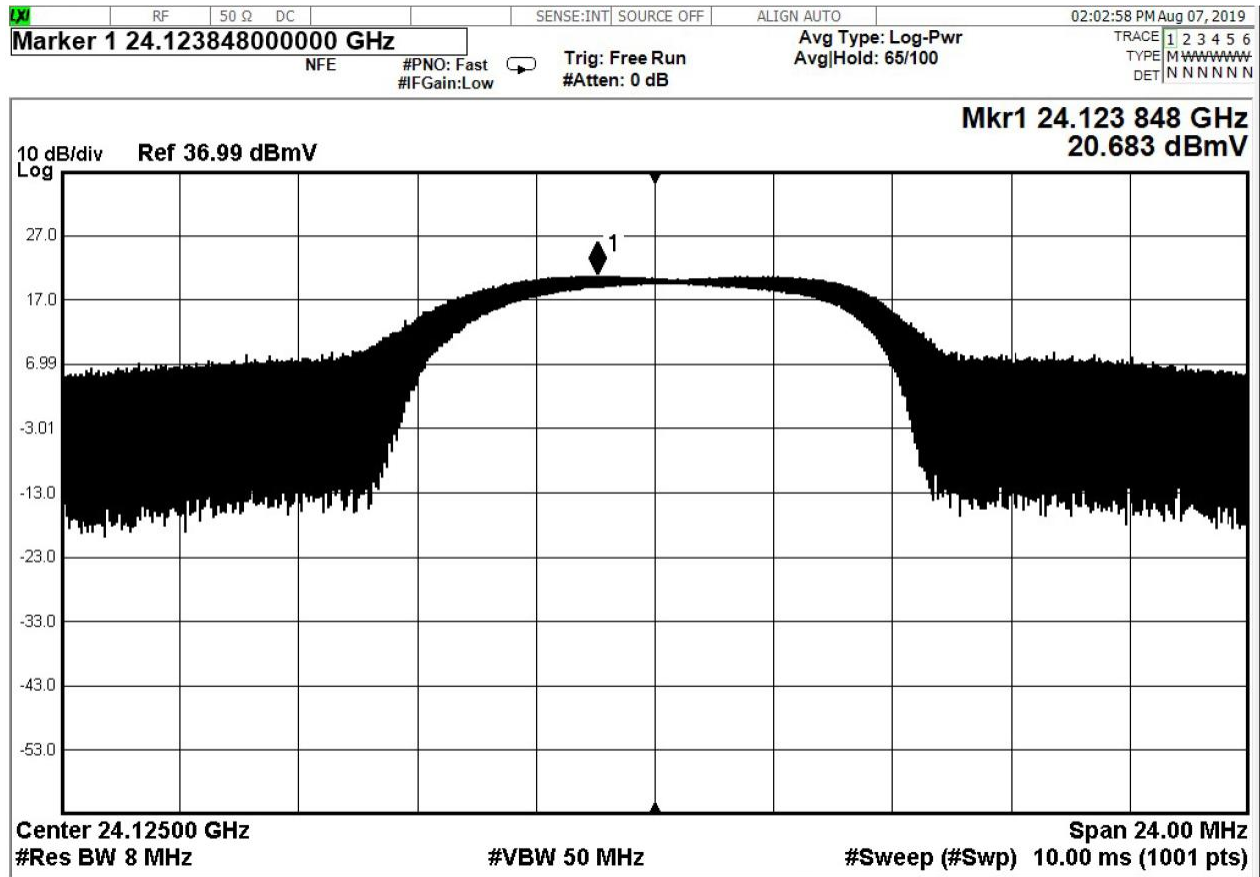
Figure 6 - Analyzer Measurement – Fundamental, Channel Mid
