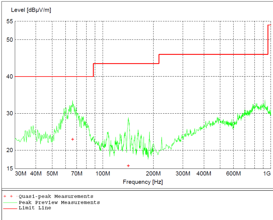
Figure 1 - Radiated Emissions Data Plot, 30M-1GHz, Receive mode
