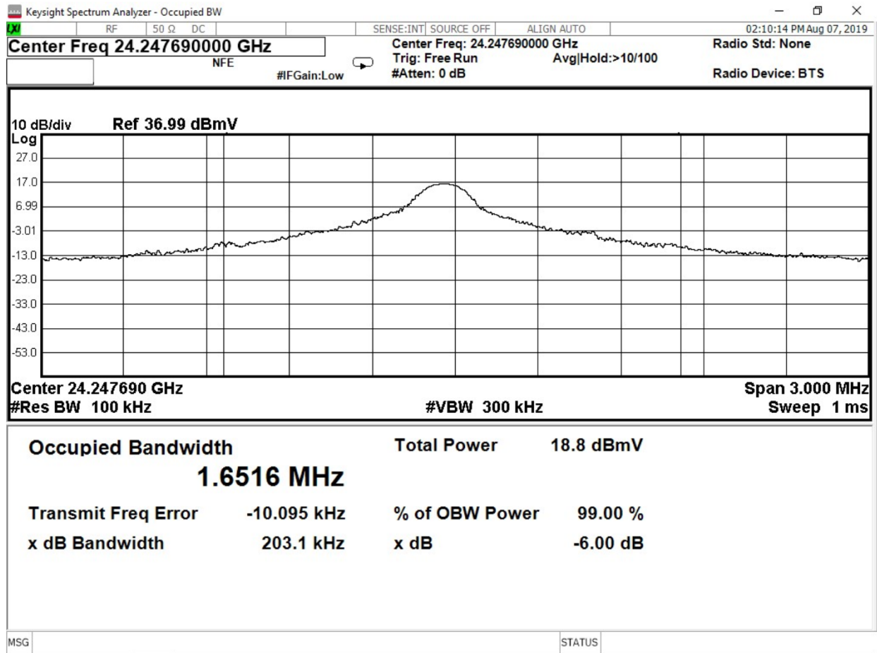
Figure 10 – Occupied Bandwidth, High channel Uncorrected measurement as recorded on spectrum analyzer
