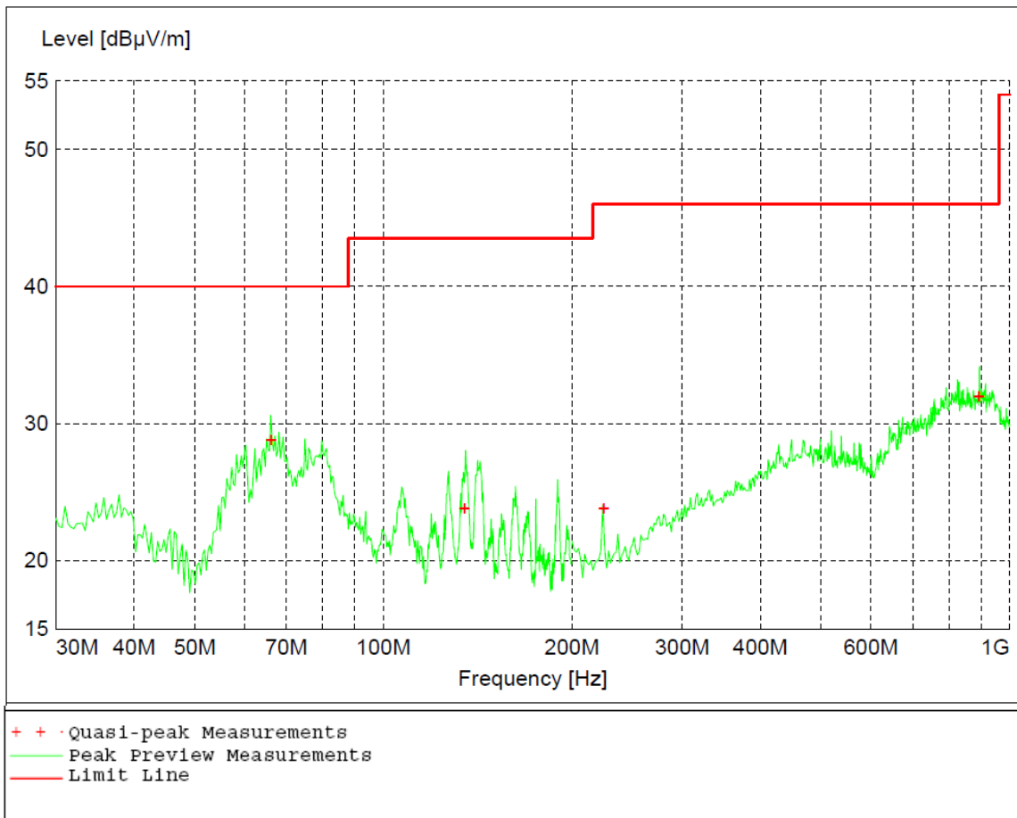
Figure 2 - Radiated Emissions Data Plot, 30M-1GHz, Low Channel
