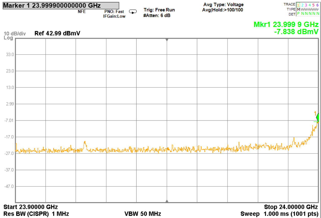
Figure 8 – Lower Band Edge, 24.00 GHz
