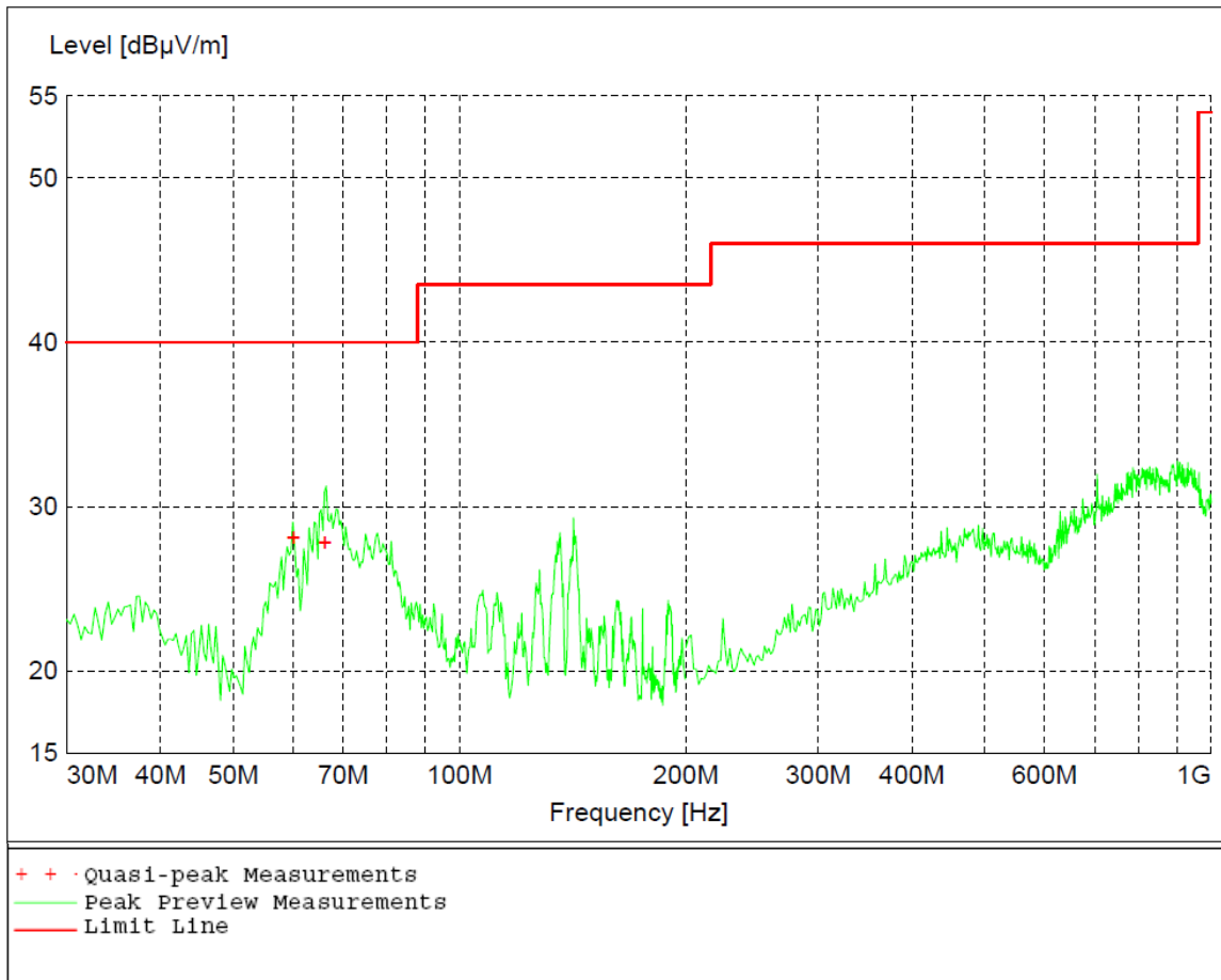
Figure 3 - Radiated Emissions Data Plot, 30M-1GHz, Mid Channel
