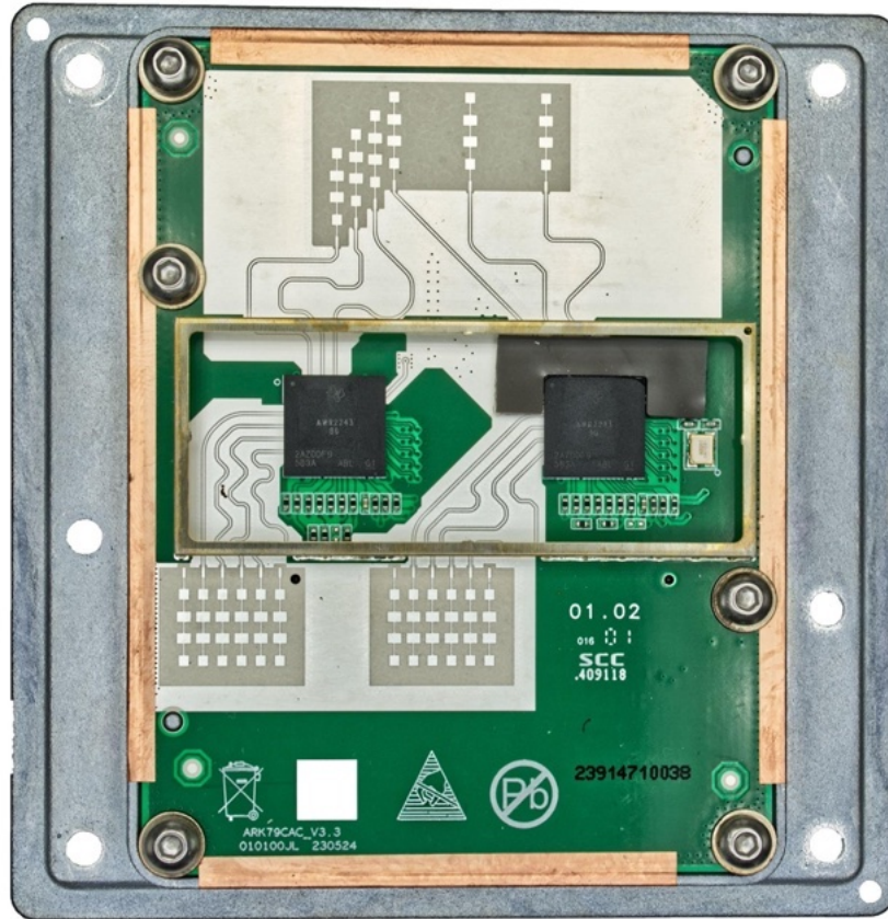
Image 16: RF board installed in unit with shielding tape and foam added.
