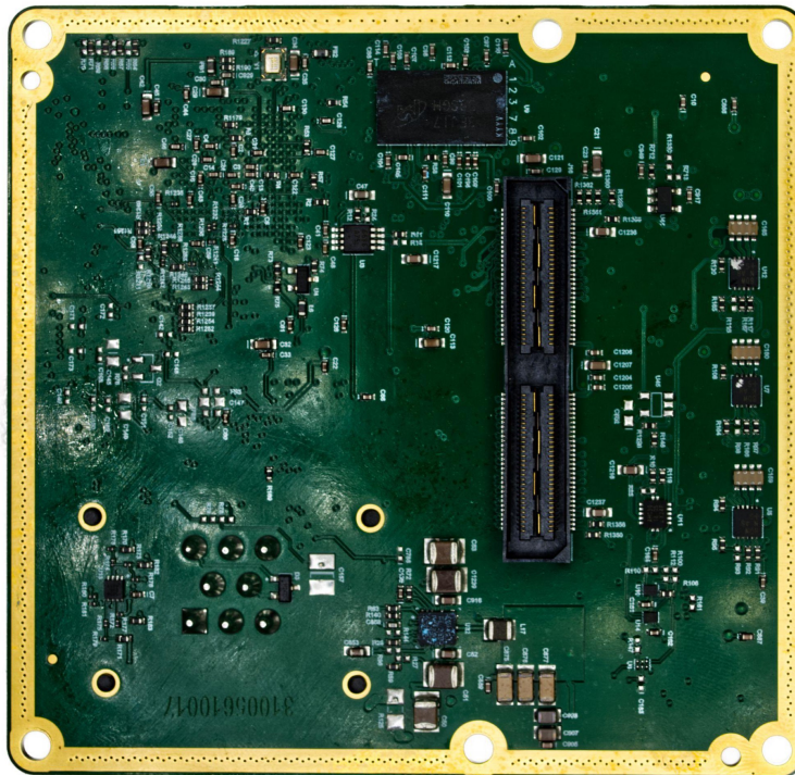
Image 20: Digital Board Front (Top)
