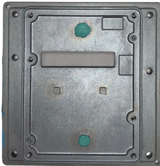
Image 11: RF Mounting Plate front side
