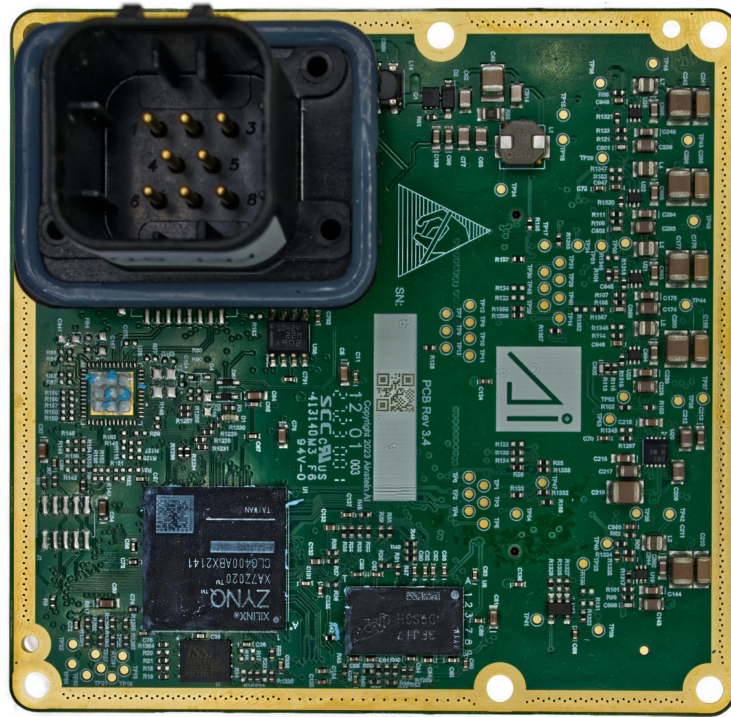
Image 19: Digital Board Back (Back of product)
