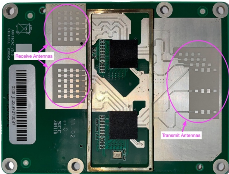
Image 15: RF Board Front - Antennas highlighted
