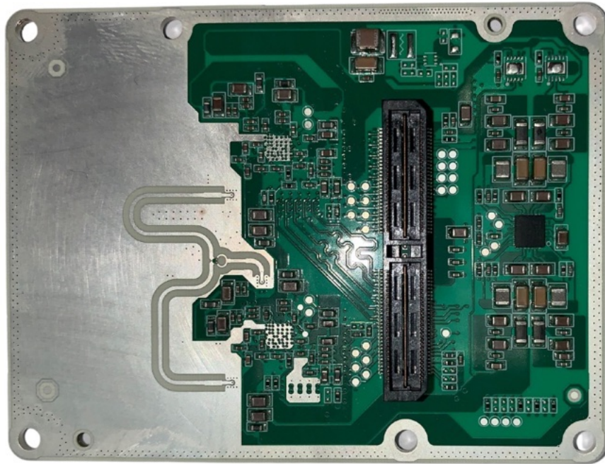
Image 14: RF Board back
