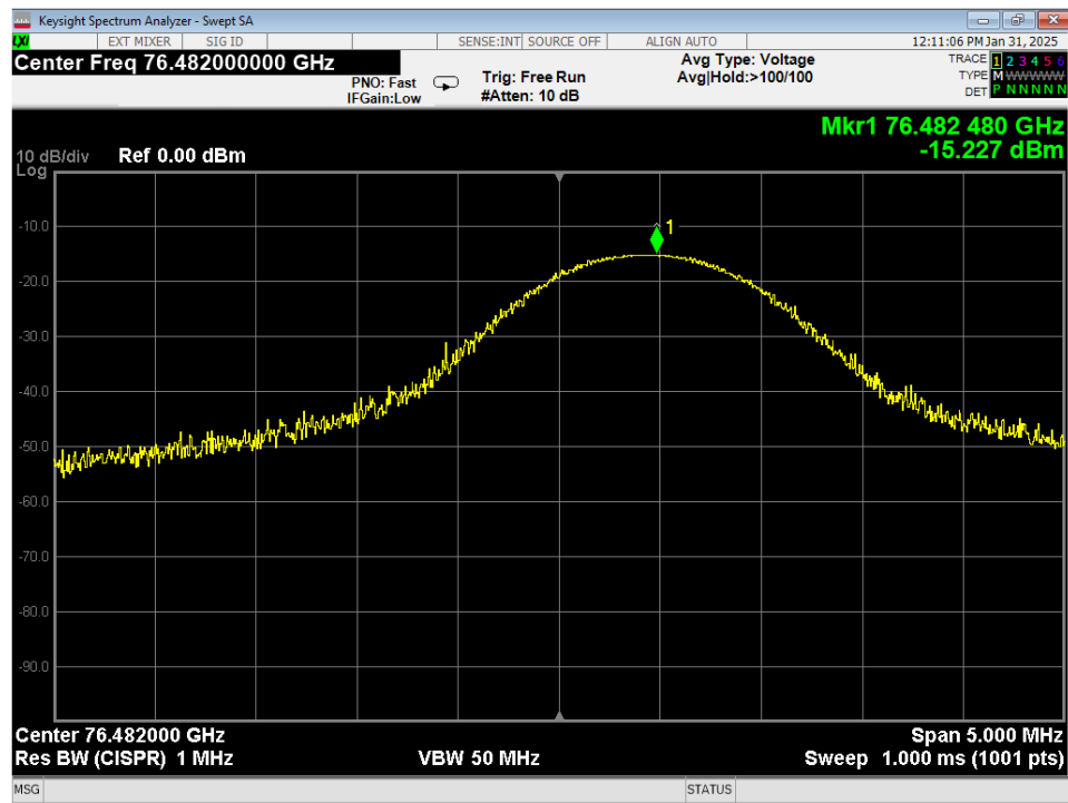
Figure 6 - Analyzer Measurement – Fundamental, High Channel
