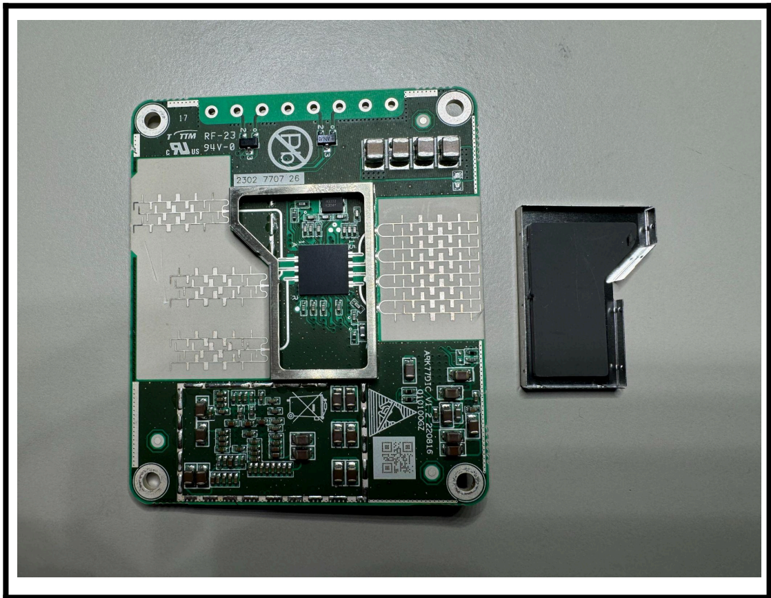
PCB Back End with Shield Off Photo
