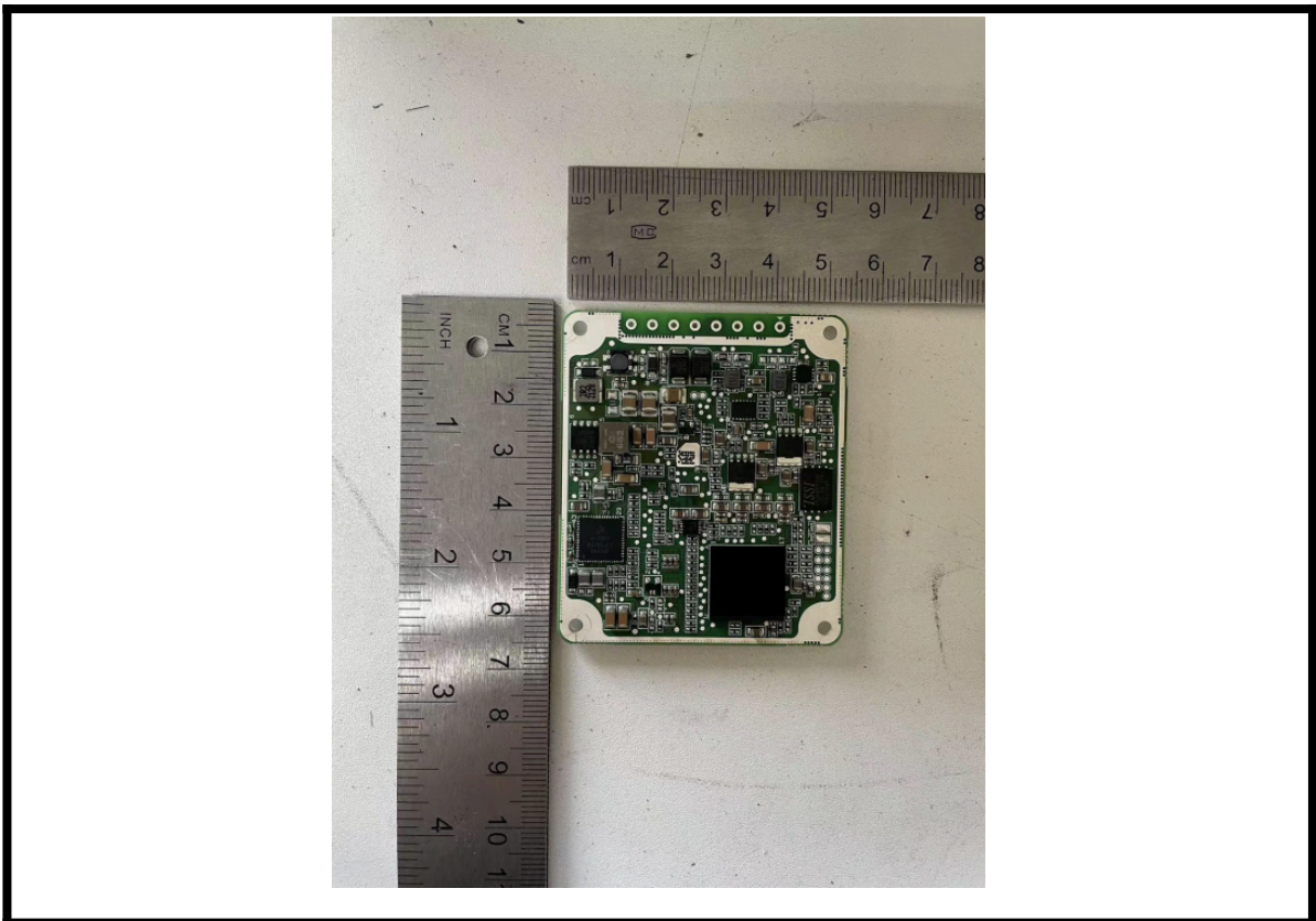
PCB Front End Photo
