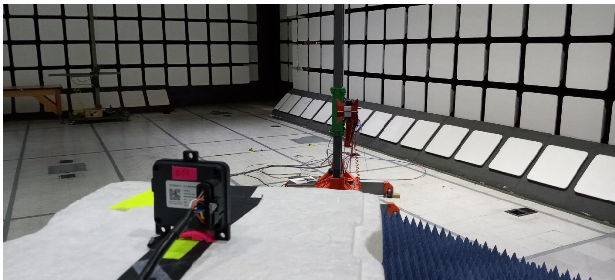
1 – 18 GHz Test Setup
