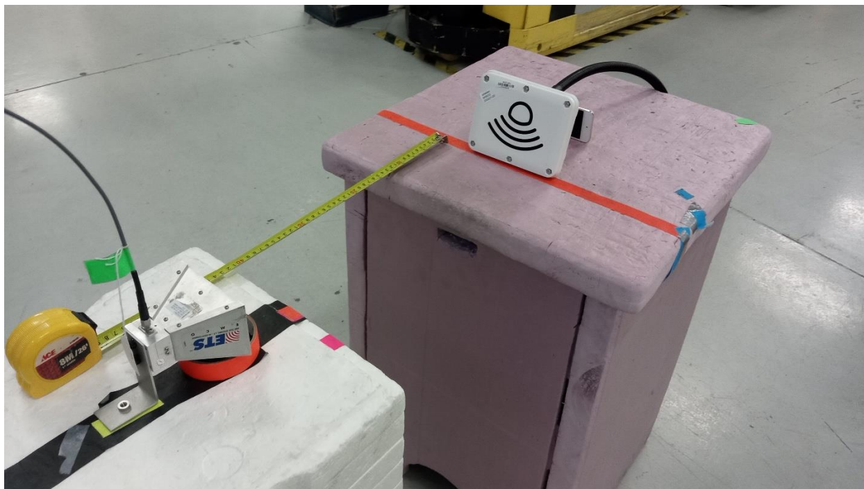
18-40 GHz Test Setup
