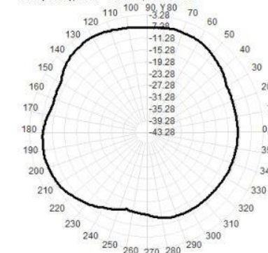
Total(H-XY), Max=-5.85dBi, CirD=10.42
