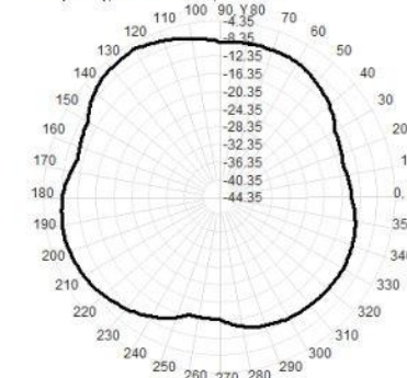
Total(H-XY), Max=-5.68dBi, CirD=11.32
