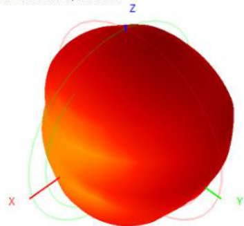
2400.0MHz H+V, Eff: 12.5%
