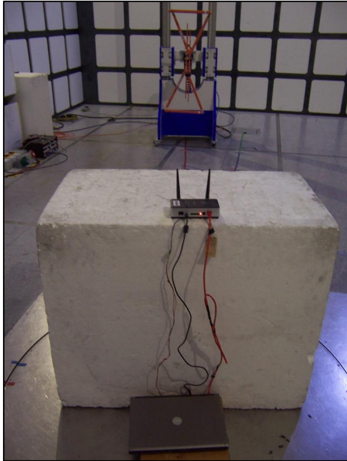
Figure 3 – 30 MHz to 5 GHz (Reader)
