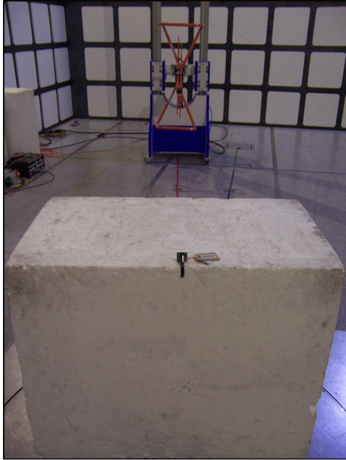
Figure 1 – 30 MHz to 1 GHz (Tag)
