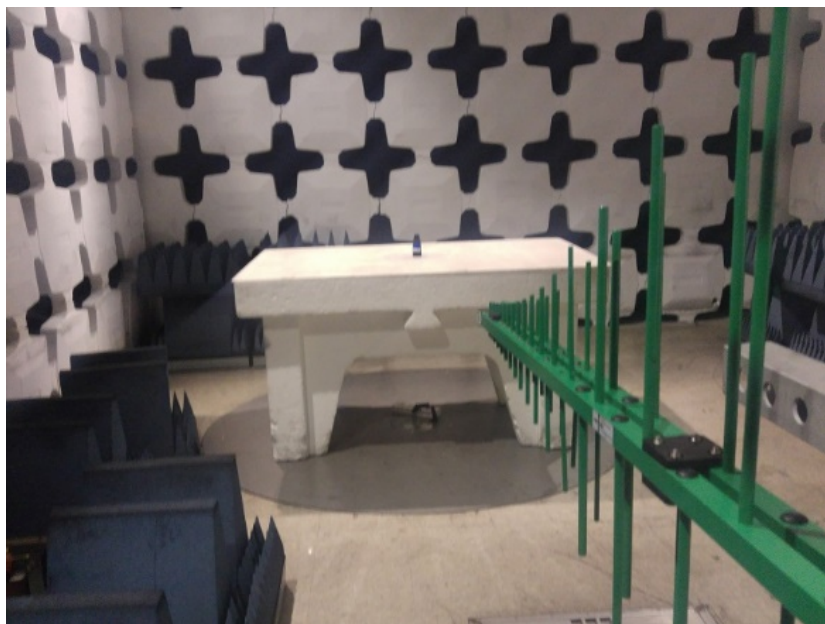
Photo 2. Radiated emissions test setup with Biconilog antenna.
