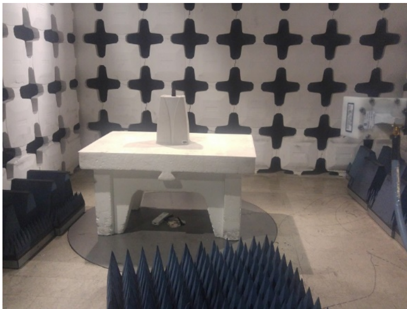
Photo 4. Radiated emissions test setup with Horn antenna in 18-25GHz.
