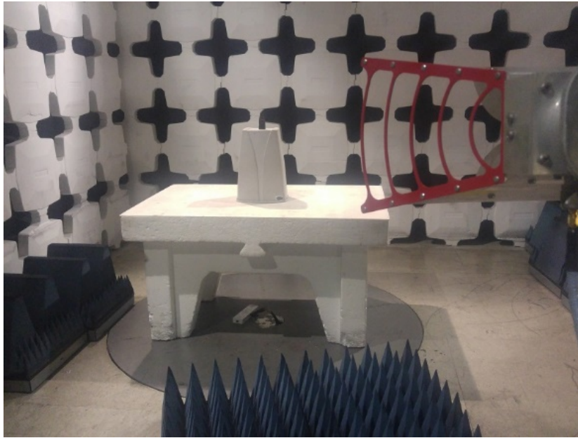
Photo 3. Radiated emissions test setup with Horn antenna in 1-18GHz.
