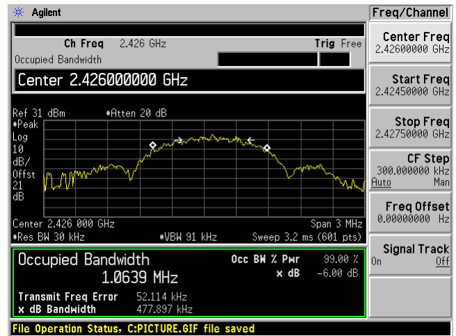
Middle Channel 2426 MHz
