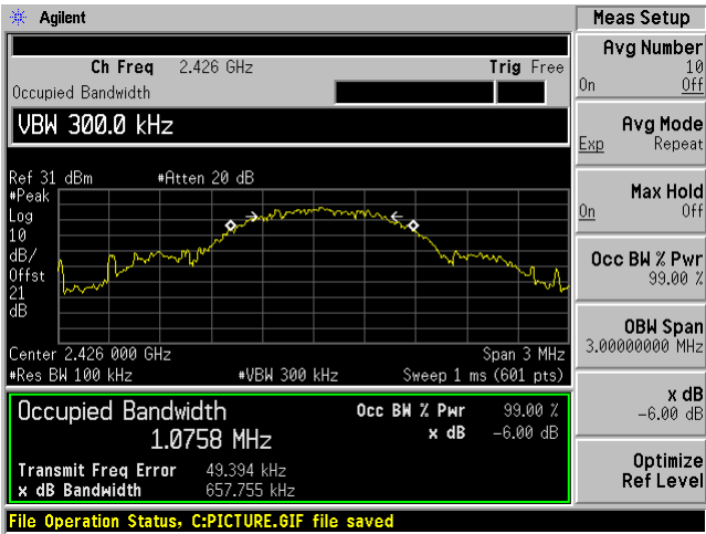
Middle Channel 2426 MHz
