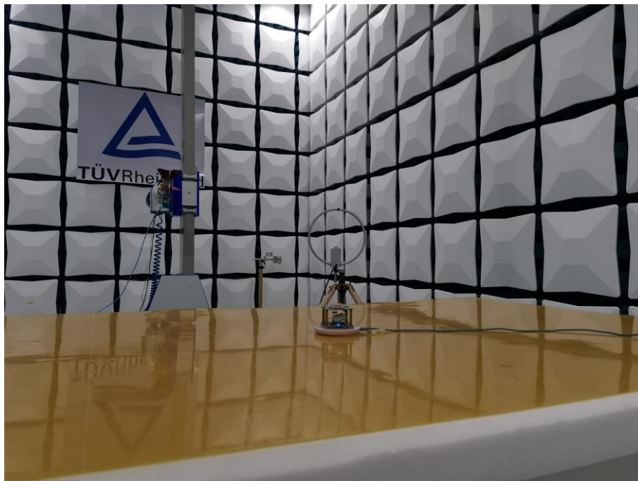
Photograph 4: Set-up for Radiated Spurious Emission
