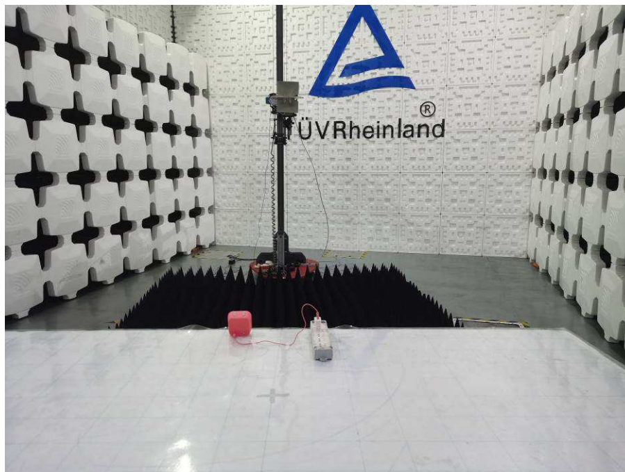
Photograph 5: Set-up photo for Radiated Emission, Above 1GHz
