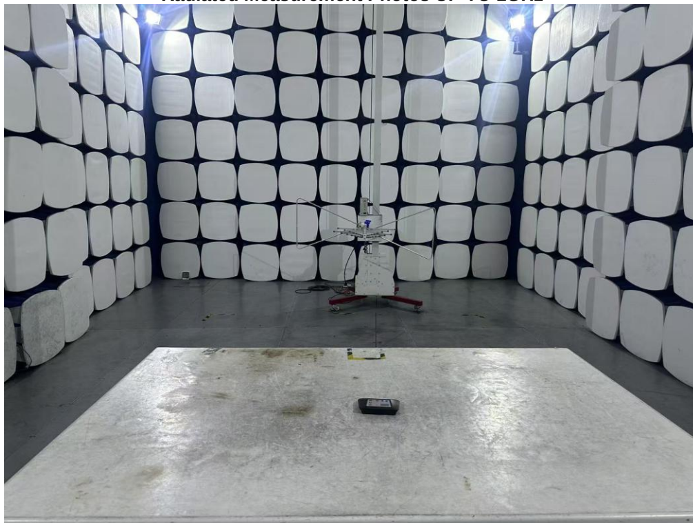
Radiated Measurement Photos UP TO 1GHz
