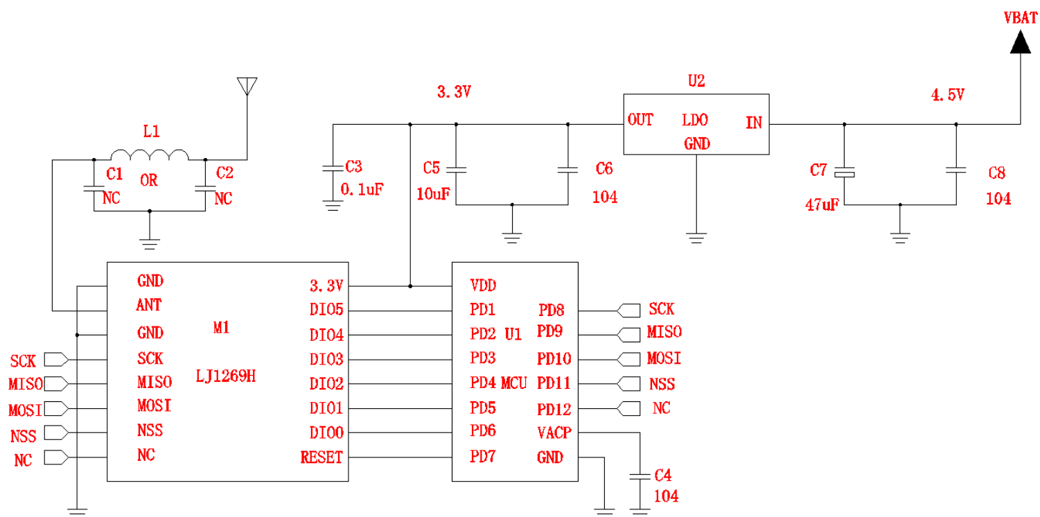
Figure 40. Typical Application Schematic
