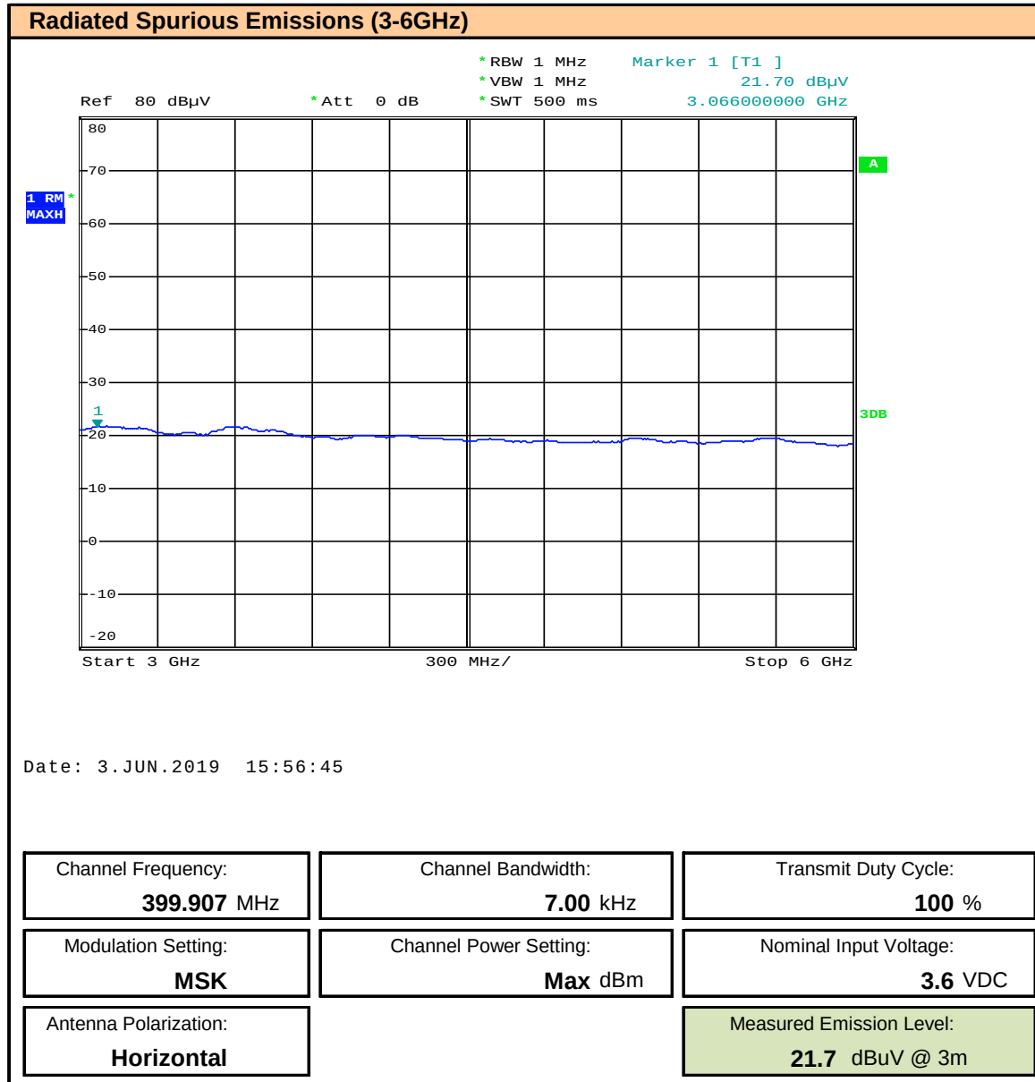
Plot 10.7 – Radiated Spurious Emissions, 3-6GHz, Horizontal
