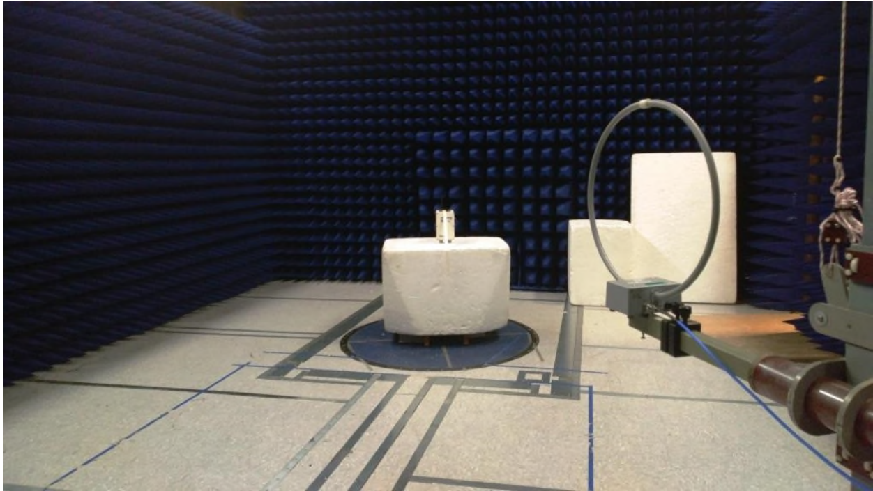
Figure 1: Equipment Under Test – Radiated Emissions <30MHz
