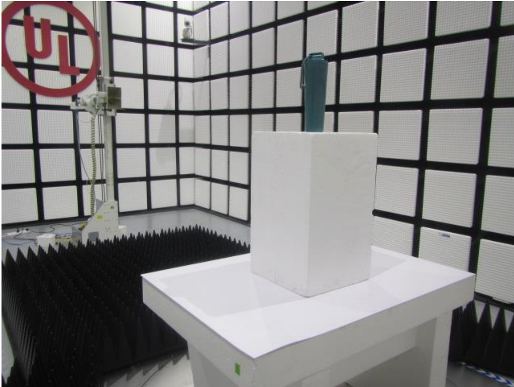
RADIATED RF MEASUREMENT ABOVE 1GHZ SETUP (Z axis)
