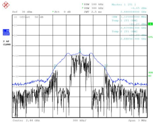
PRBS9: 99% bandwidth on Channel 0
