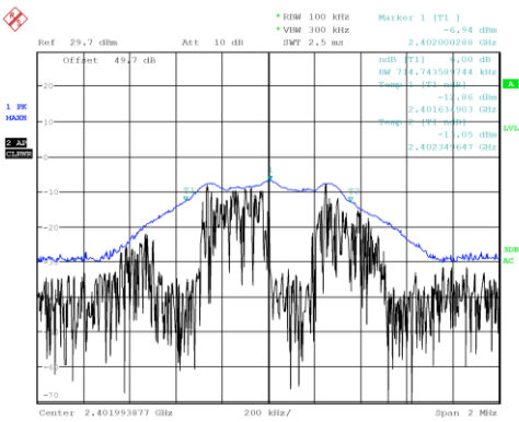
PRBS9 : 6 dB bandwidth on Channel 0
