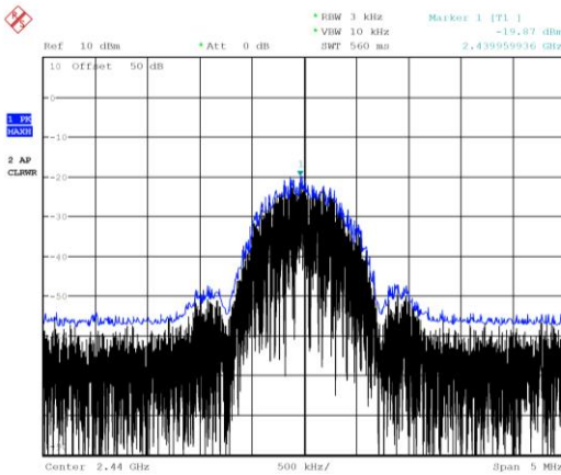
Middle channel, vertical polarization
