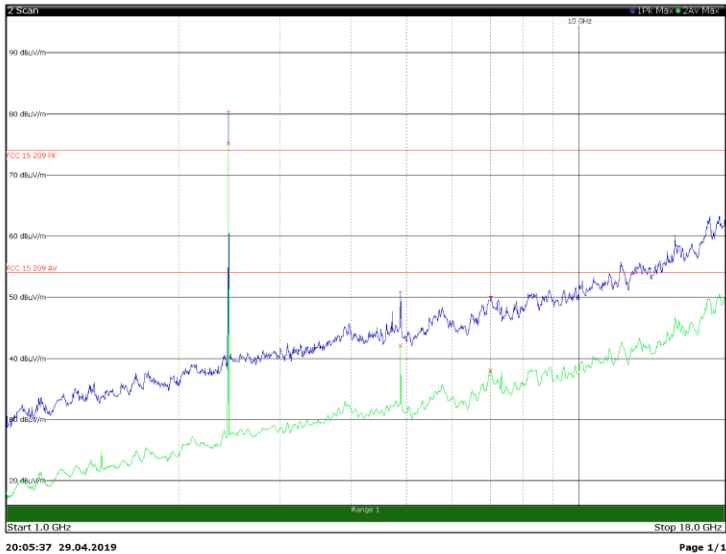
Section 8 Radiated measurement BT horizontal polarization middle channel
