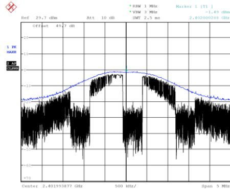
Channel 0, vertical polarization
