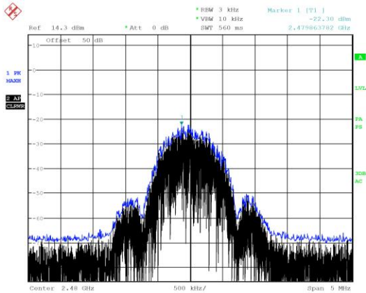
High channel, vertical polarization
