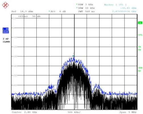
High channel, horizontal polarization
