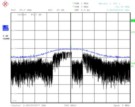
Channel 0, horizontal polarization
