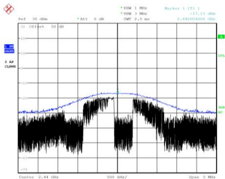
Middle channel, horizontal polarization
