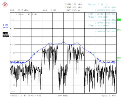
PRBS9: 99% bandwidth on Channel 0
