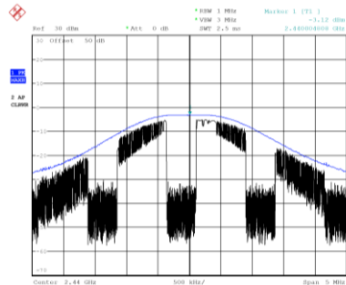
Middle channel, vertical polarization
