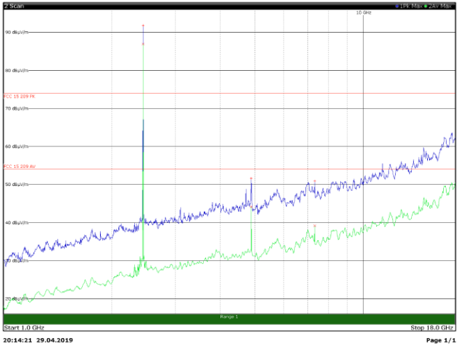
Section 8 Radiated measurement BT vertical polarization Middle channel
