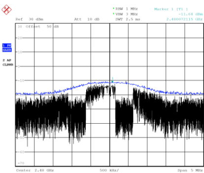
High channel vertical polarization
