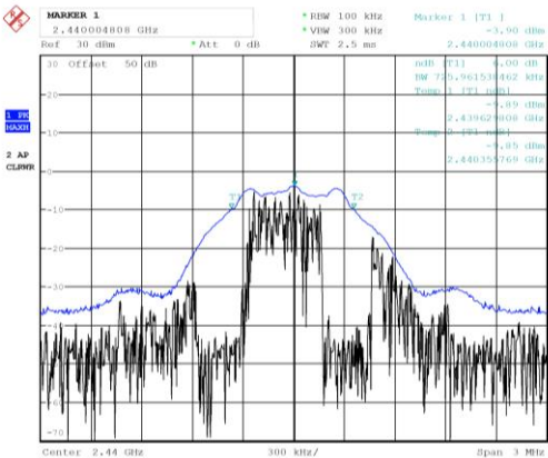
PRBS9 : 6 dB bandwidth on Channel 0
