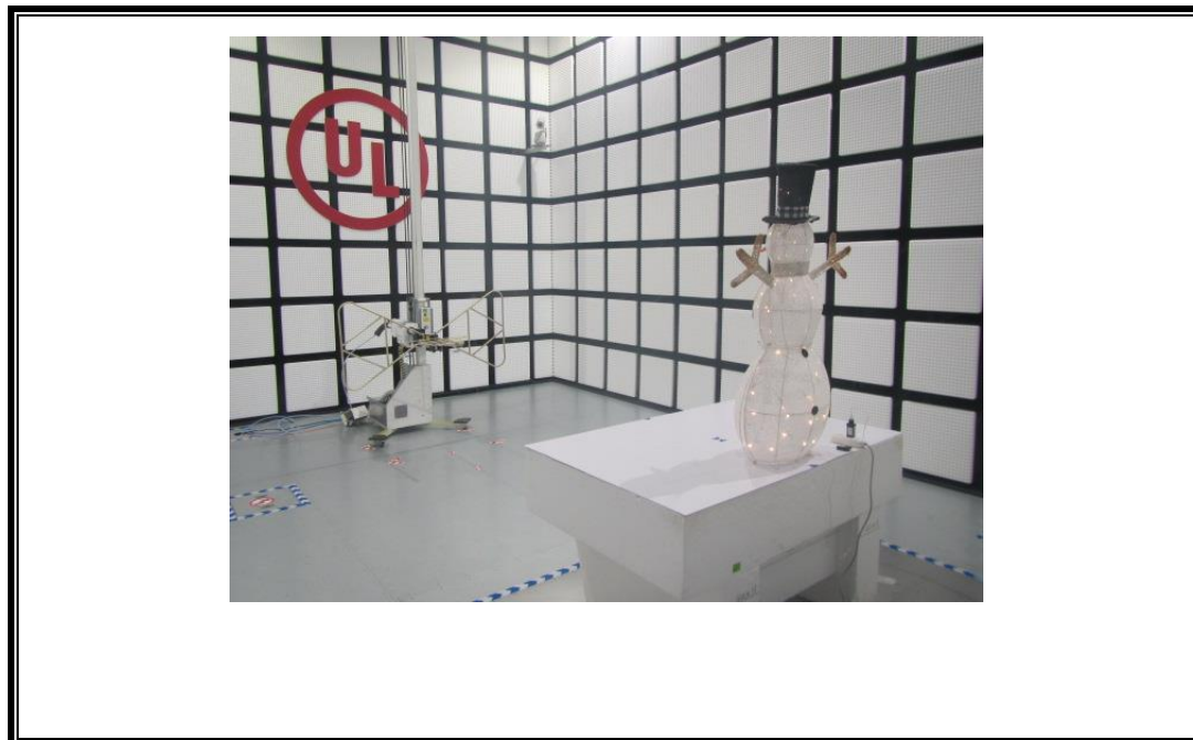
Radiated Disturbance below 1GHz (Side)
