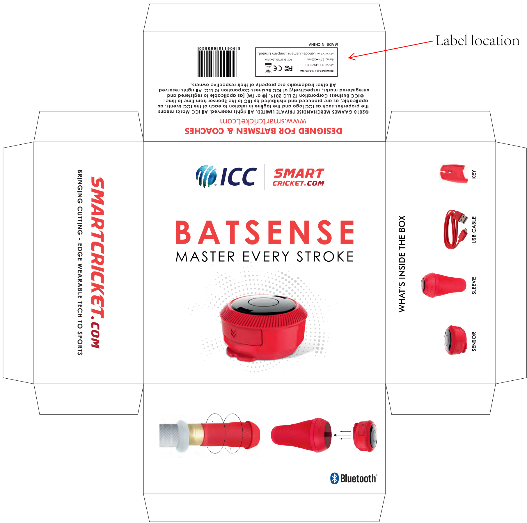
BOX COVER DESIGN (mounting on 2.5mm cardboard)
