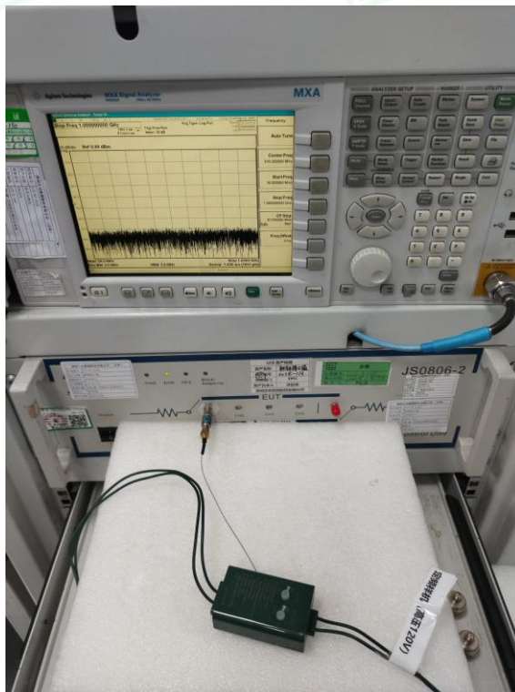
Test Setup Photo of RF Conducted
