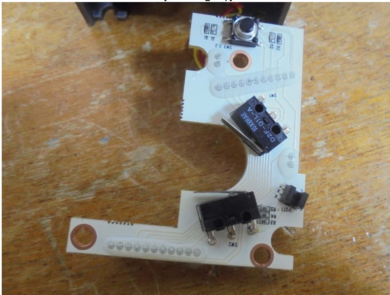
[Sub Board_2 Top]
