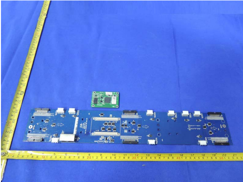
Solder Board-Component View 8
