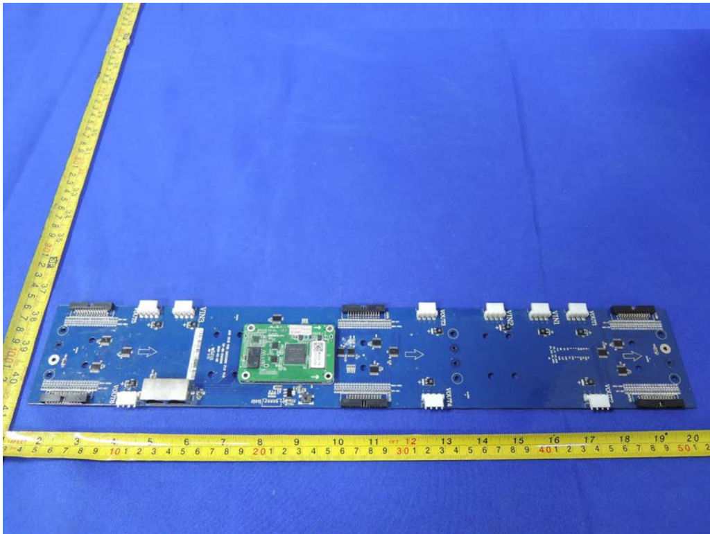
Solder Board-Component View 6
