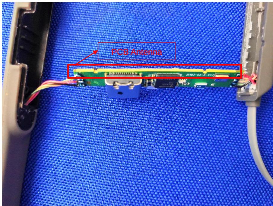
ANTENNA CLOSE-UP 1
