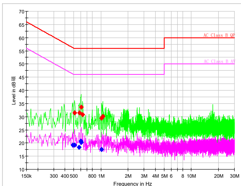
L+N Line
