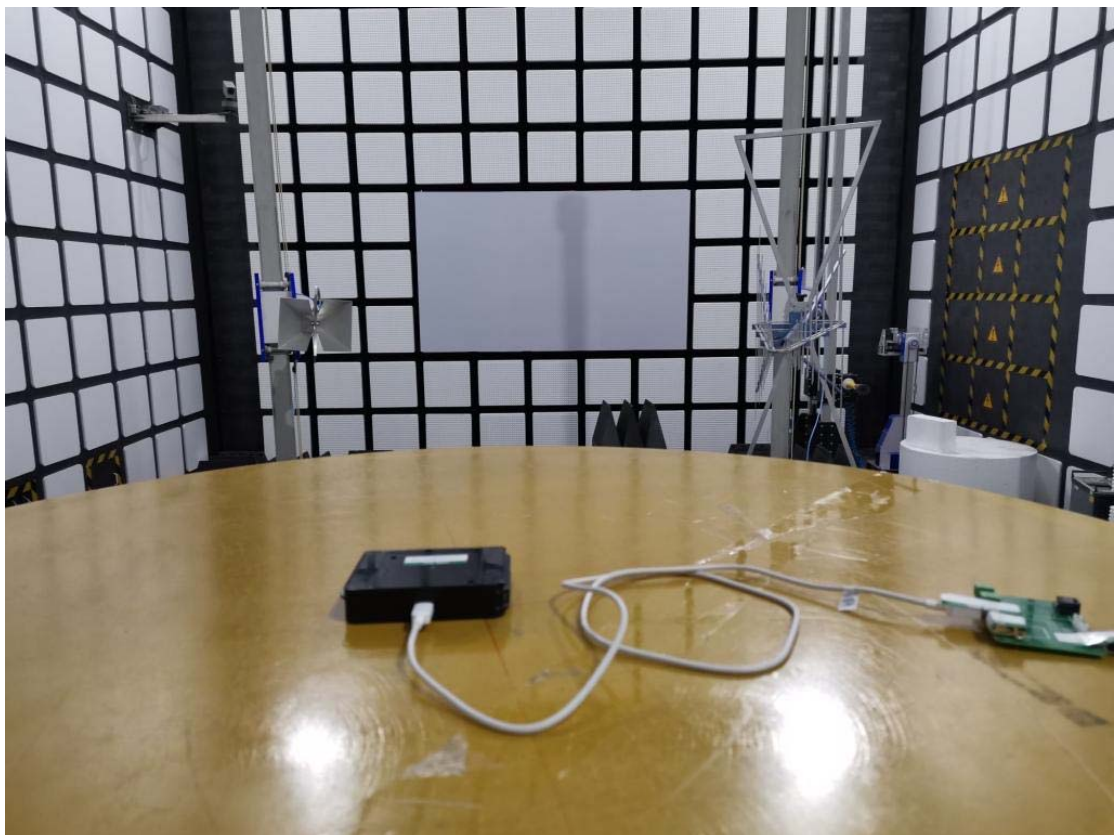
Radiated test setup
