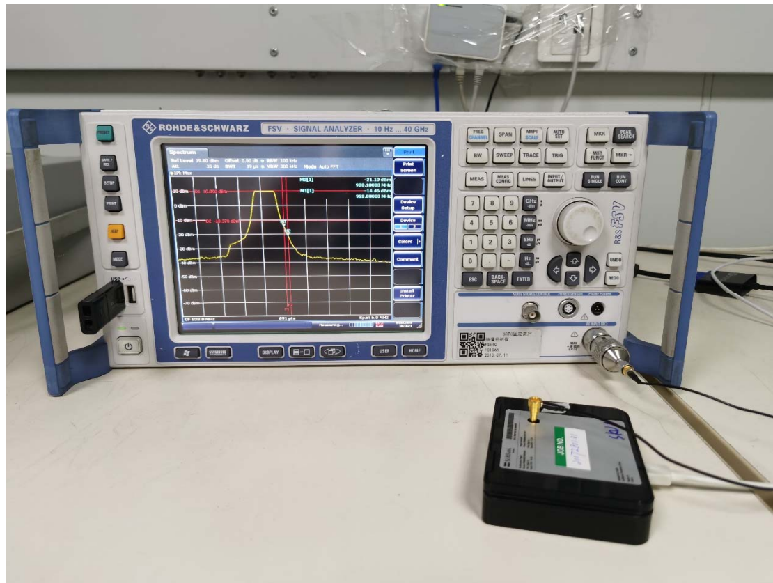
Conducted test setup
