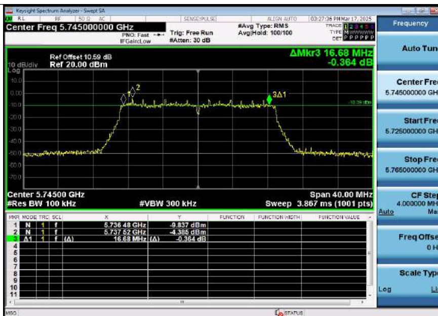
11N20SISO-Ant1-5745-PASS
