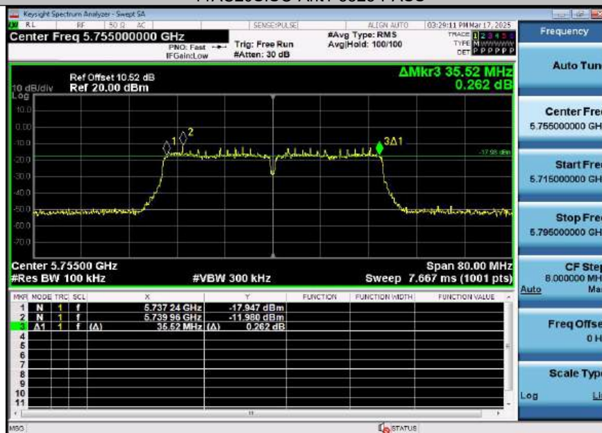
11AC40SISO-Ant1-5755-PASS
