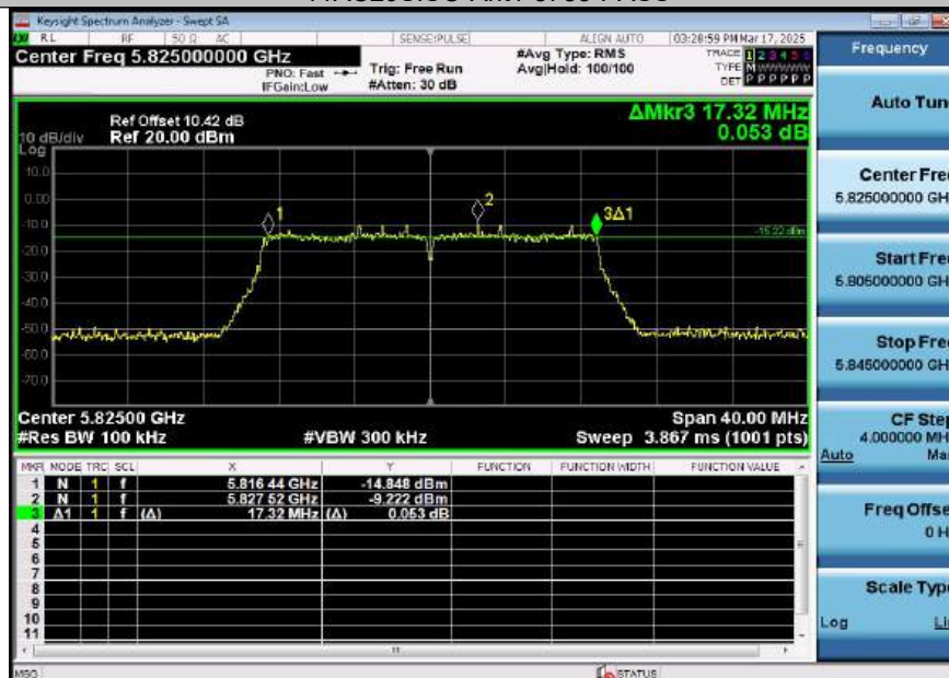
11AC20SISO-Ant1-5825-PASS
