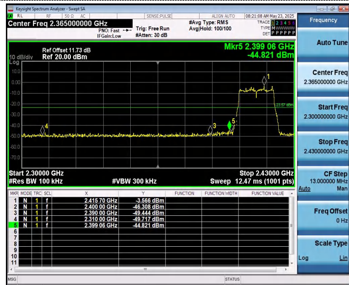
Left bandedge
