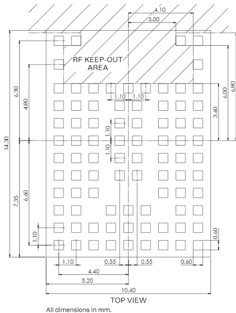
Figure 16: MAYA-W2 footprint
