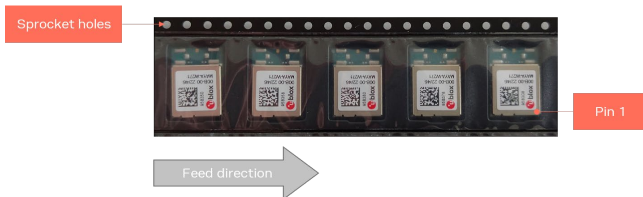
Figure 23: Orientation of MAYA-W2 modules on tape
