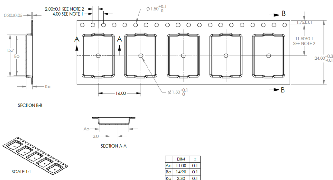
Figure 24: MAYA-W2 tape dimensions
