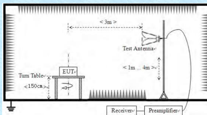
Above 1GHz
