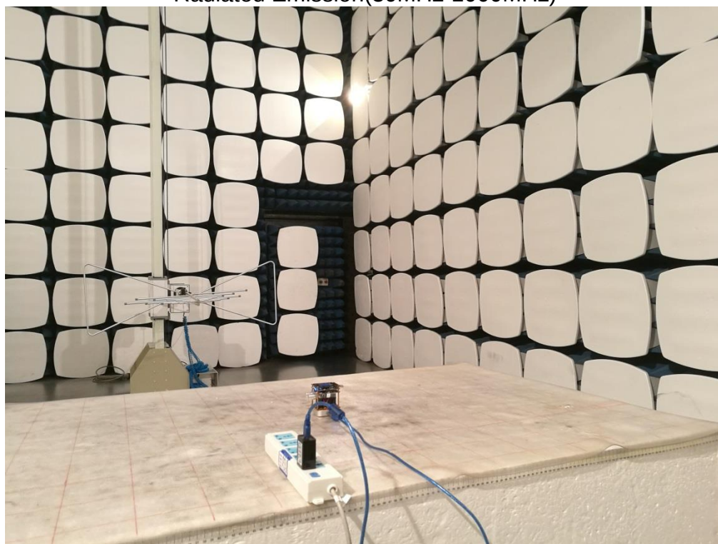
Radiated Emission(30MHz-1000MHz)
