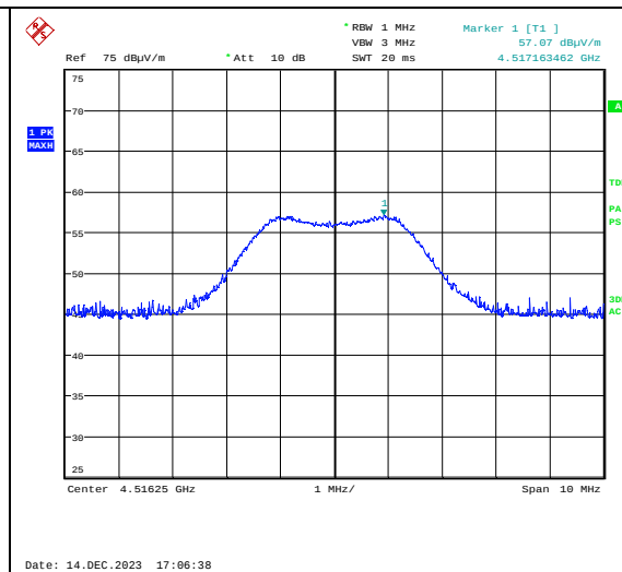
Emissions 4516.25 MHz, 903.25 MHz, Max: HP
