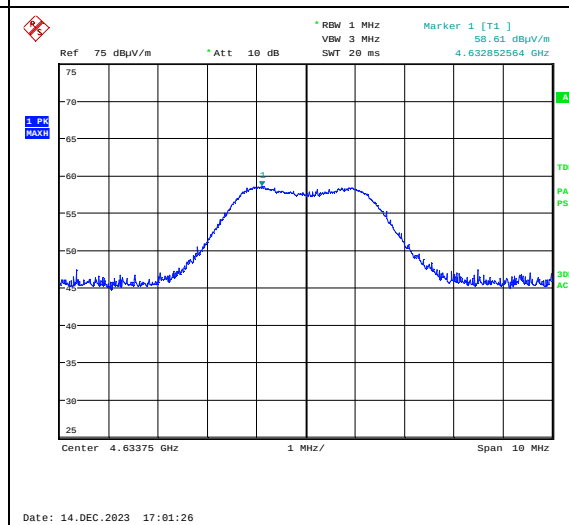
Emissions 4633.75 MHz, 926.75 MHz, Max: HP
