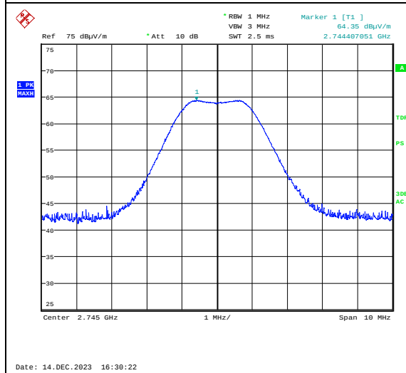
Emissions 2745.00 MHz, 915.00 MHz, Max: VP
