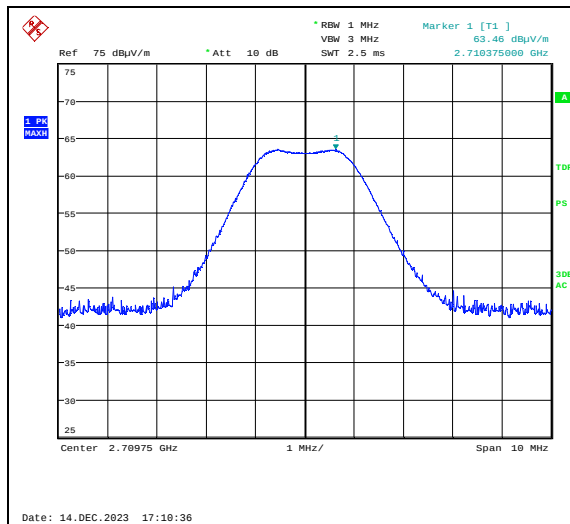
Emissions 2709.75 MHz, 903.25 MHz, Max: VP
