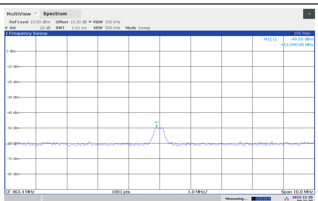
Conducted Emissions 463.4 MHz, 926.75 MHz
