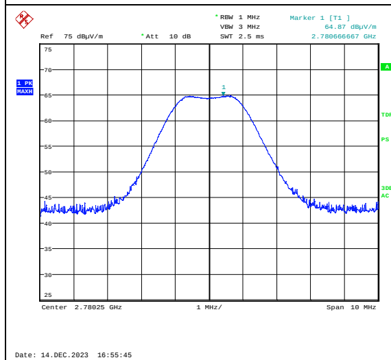
Emissions 2780.25 MHz, 926.75 MHz, Max: VP
