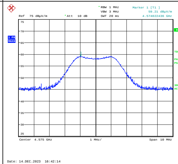
Emissions 4575.00 MHz, 915.00 MHz, Max: HP
