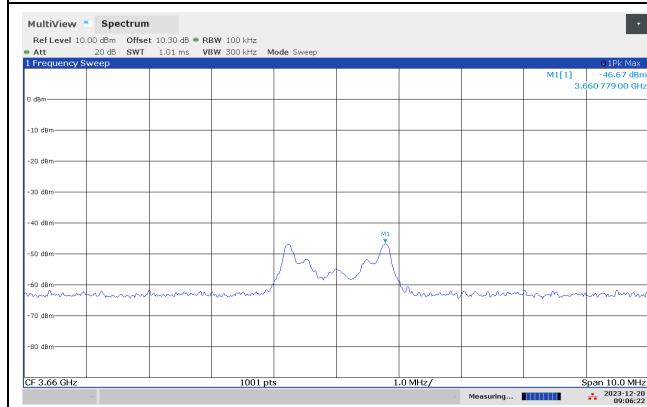
Conducted Emissions 3660 MHz, 915 MHz
