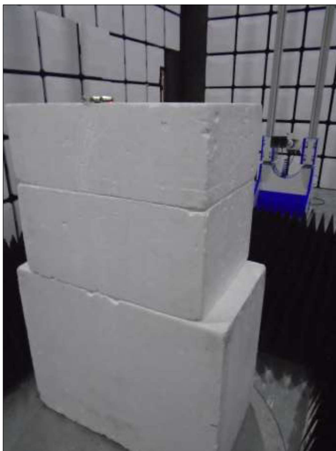
Figure 66 - Test Setup - 1 GHz to 10 GHz - X Orientation
