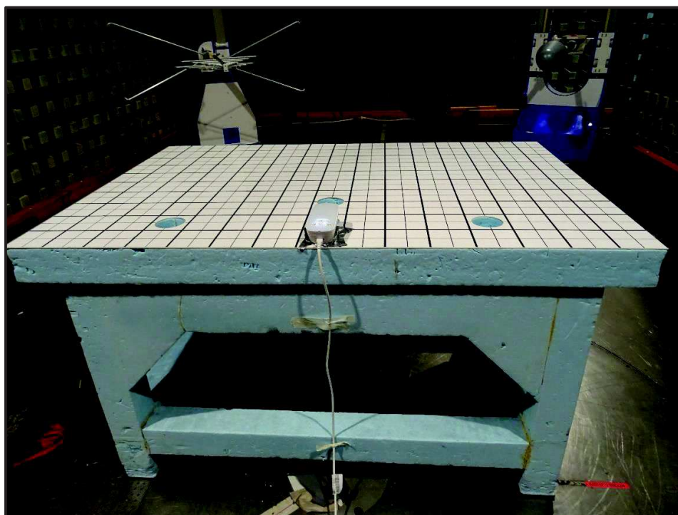
Photo 6: Radiated Test Sample-30 MHz to 1GHz EUT Laying
