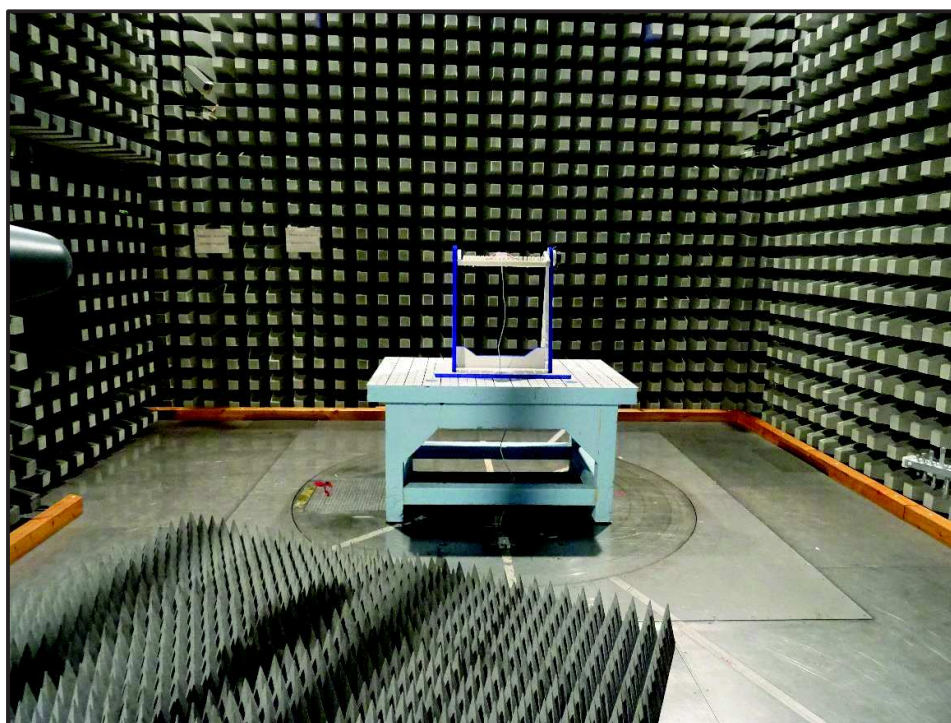
Photo 10: Radiated Test Sample-1 GHz to 10 GHz EUT Laying
