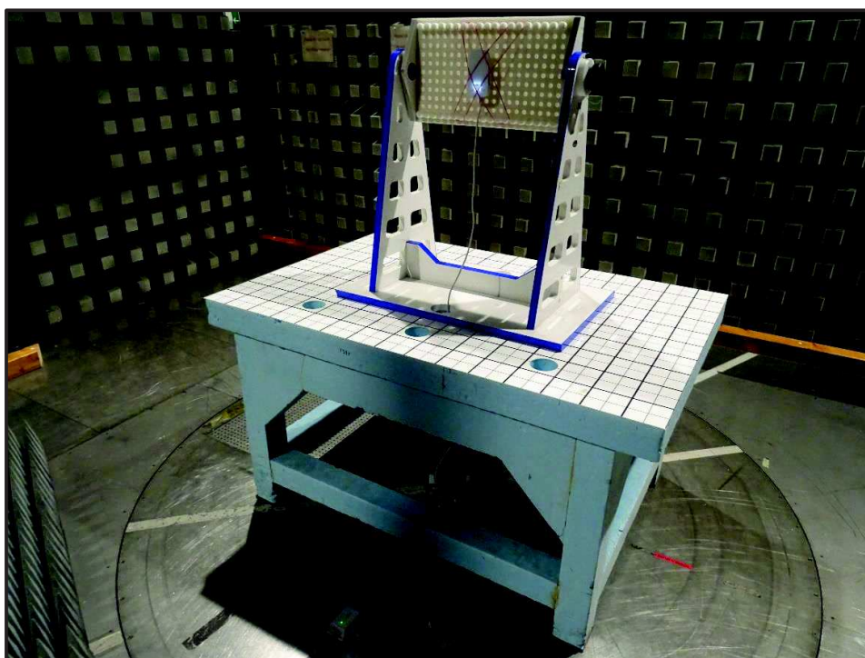
Photo 12: Radiated Test Sample-1 GHz to 10 GHz EUT Standing
