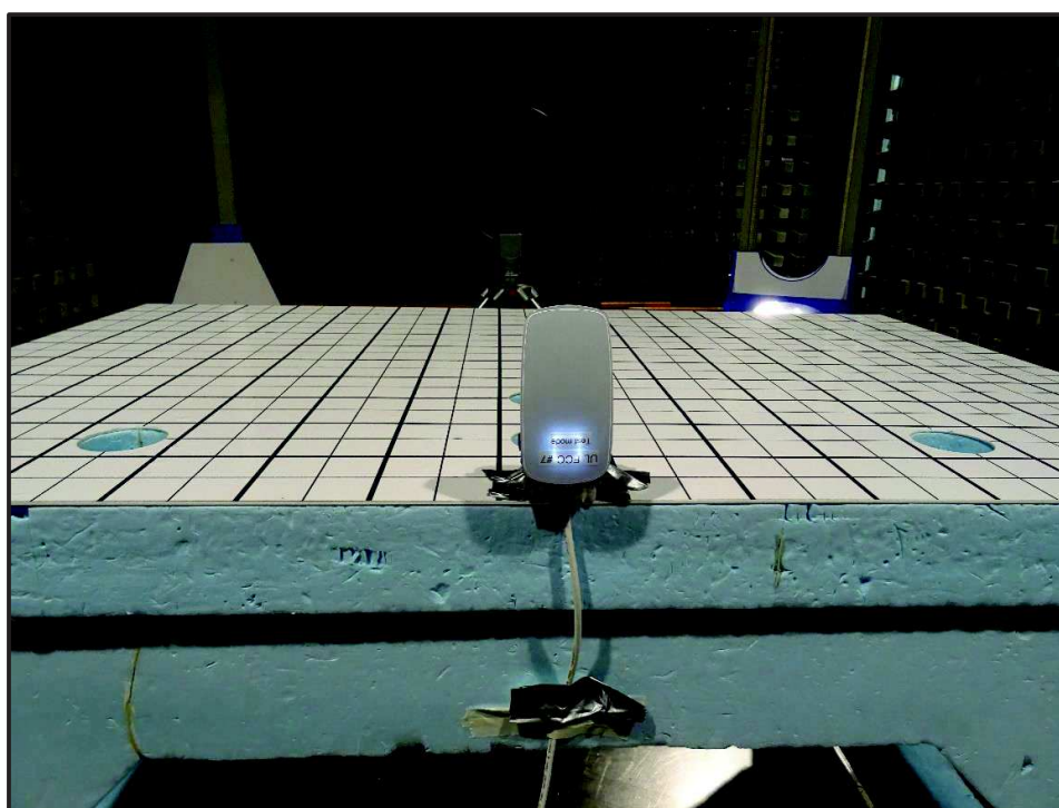
Photo 4: Radiated Test Sample-9 kHz to 30 MHz EUT Standing
