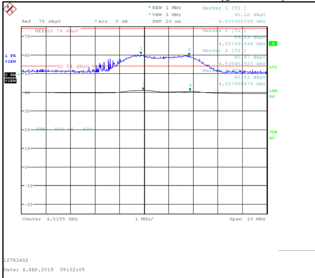
Plot: Re-Measurements for the bottom channel (@ 4.5155 GHz)
