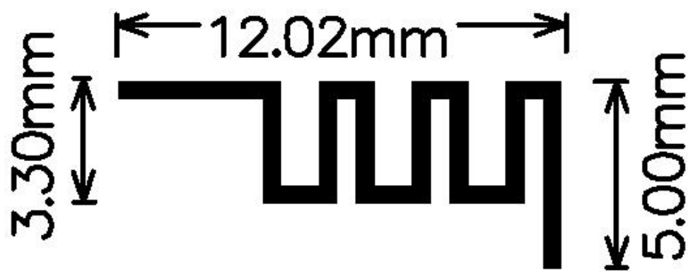
Antenna Photo & Length (mm)
