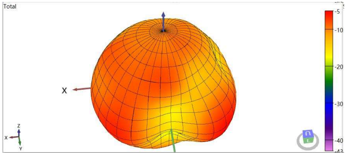
Antenna 2440MHz 3D Total Pattern
