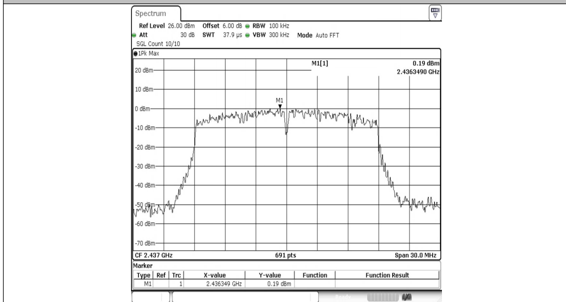
11N20MIMO-Ant1-2437-0~Reference-PASS
