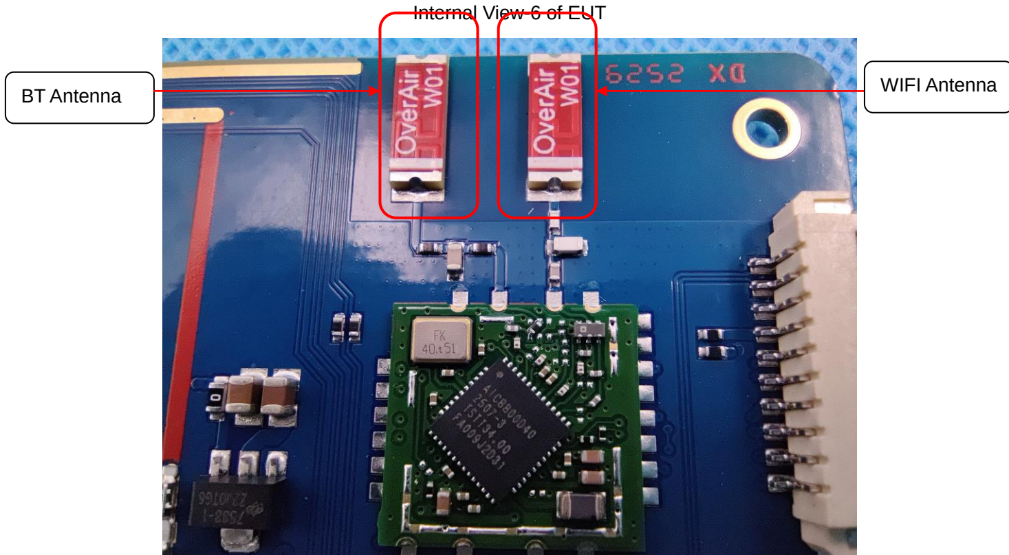
Internal View 6 of EUT
