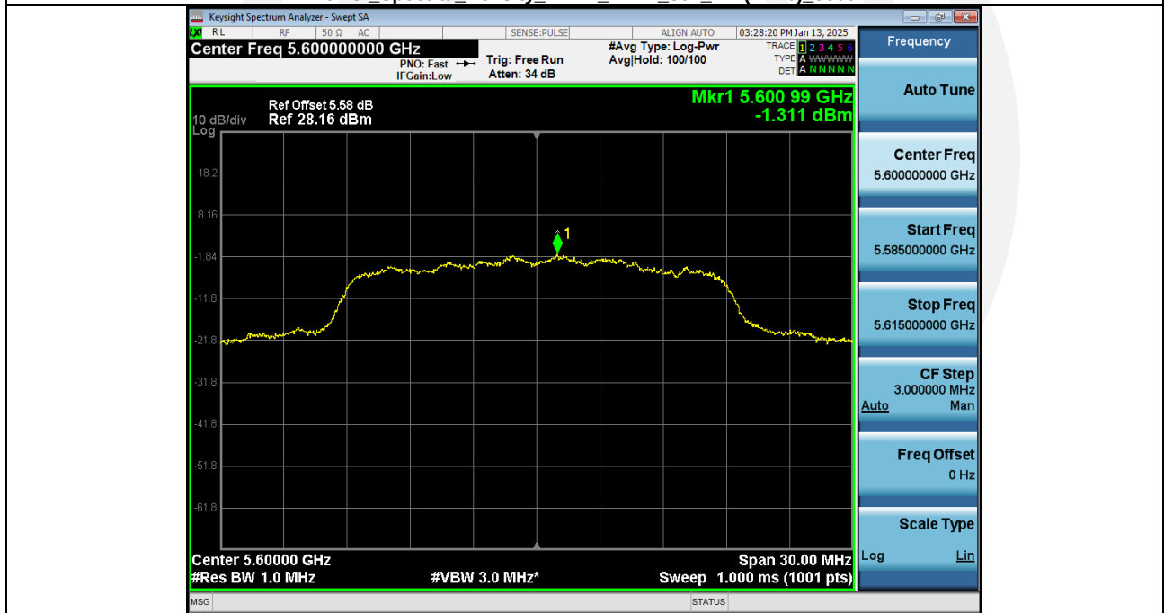
Power_Spectral_Density_NVNT_ANT2_802_11n(HT20)_5600
