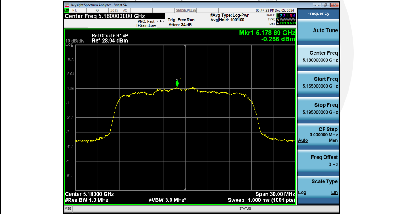
Power_Spectral_Density_NVNT_ANT2_802_11n(HT20)_5180
