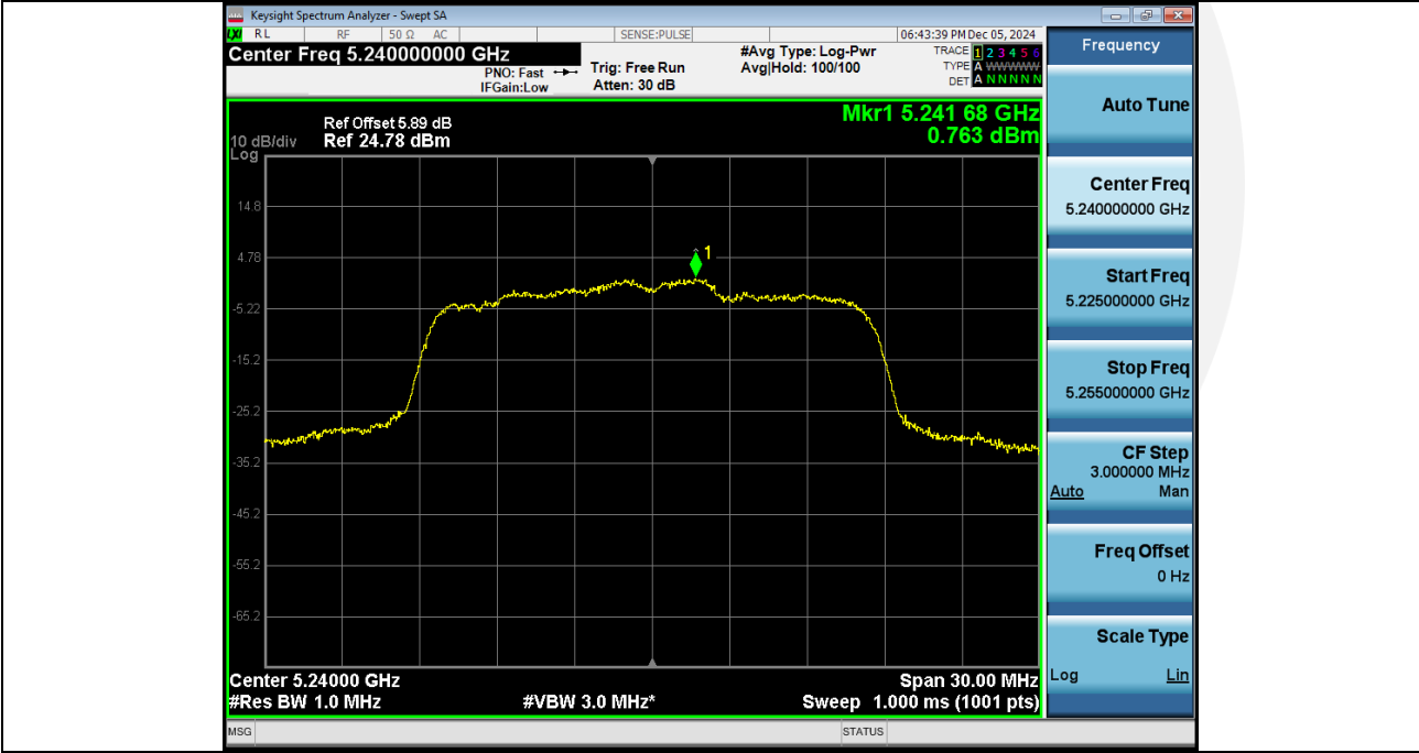
Power_Spectral_Density_NVNT_ANT2_802_11a_5240
