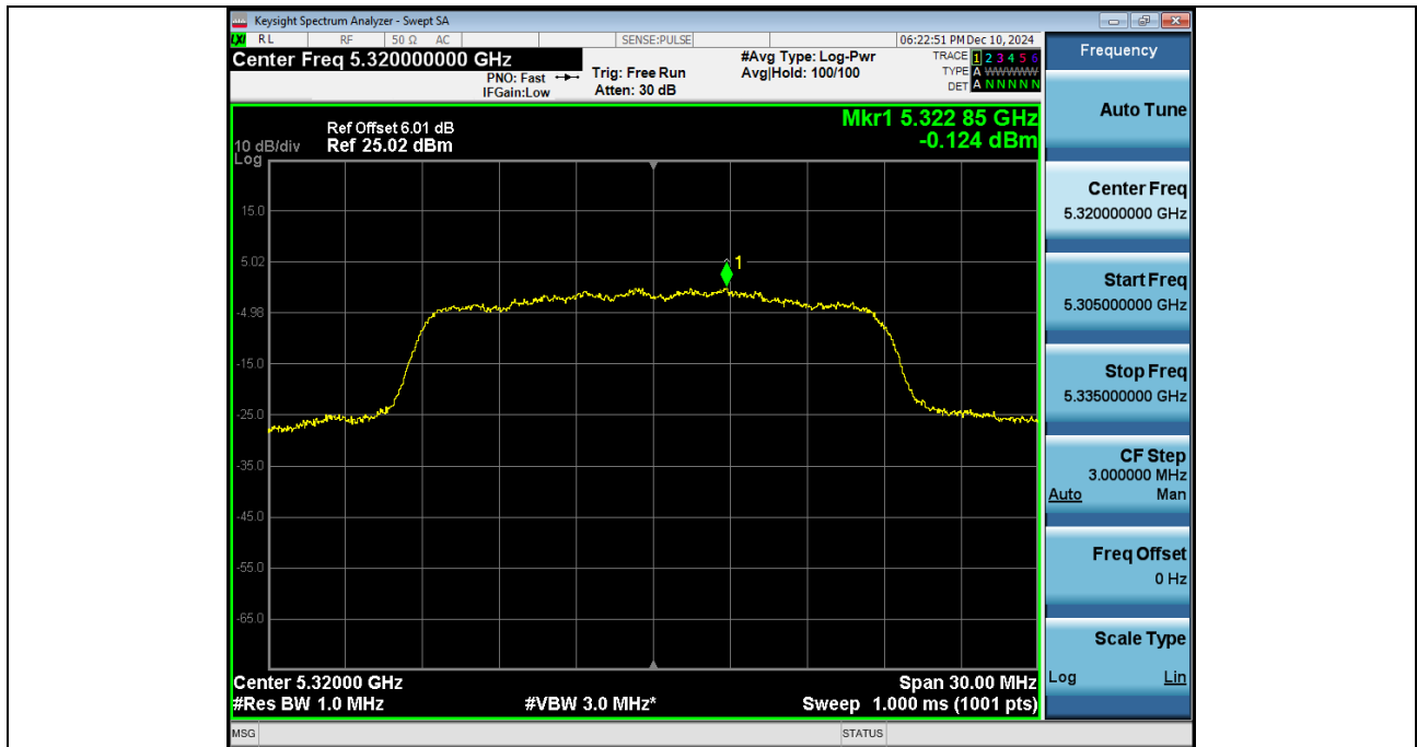
Power_Spectral_Density_NVNT_ANT2_802_11n(HT20)_5320
