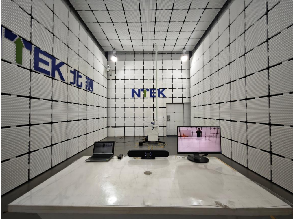
Radiated Measurement Photos(30MHz~1GHz )
